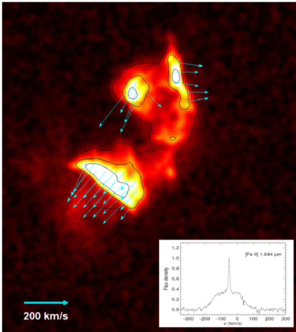
Figure 9. from Bon-Chul Koo et al 2025 Astrophys. J. Suppl. 280 doi:10.3847/1538-4365/adf0fd https://dx.doi.org/10.3847/1538-4365/adf0fd © 2025. The Author(s). Published by the American Astronomical Society.
