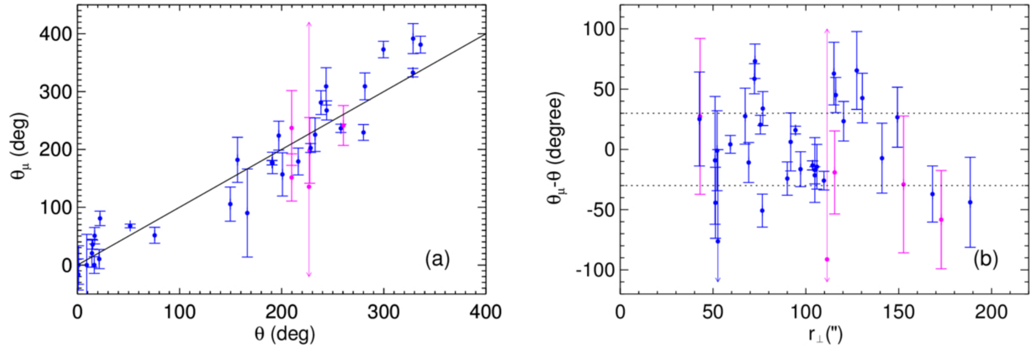
Figure 4. from Bon-Chul Koo et al 2025 Astrophys. J. Suppl. 280 doi:10.3847/1538-4365/adf0fd https://dx.doi.org/10.3847/1538-4365/adf0fd © 2025. The Author(s). Published by the American Astronomical Society.
