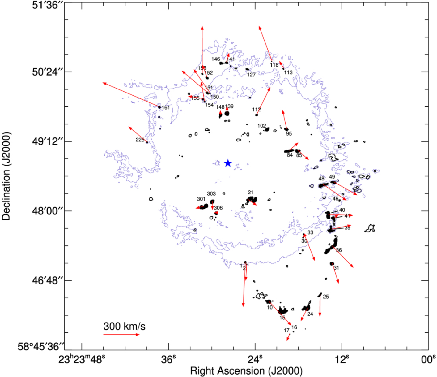
Figure 3. from Bon-Chul Koo et al 2025 Astrophys. J. Suppl. 280 doi:10.3847/1538-4365/adf0fd https://dx.doi.org/10.3847/1538-4365/adf0fd © 2025. The Author(s). Published by the American Astronomical Society.
