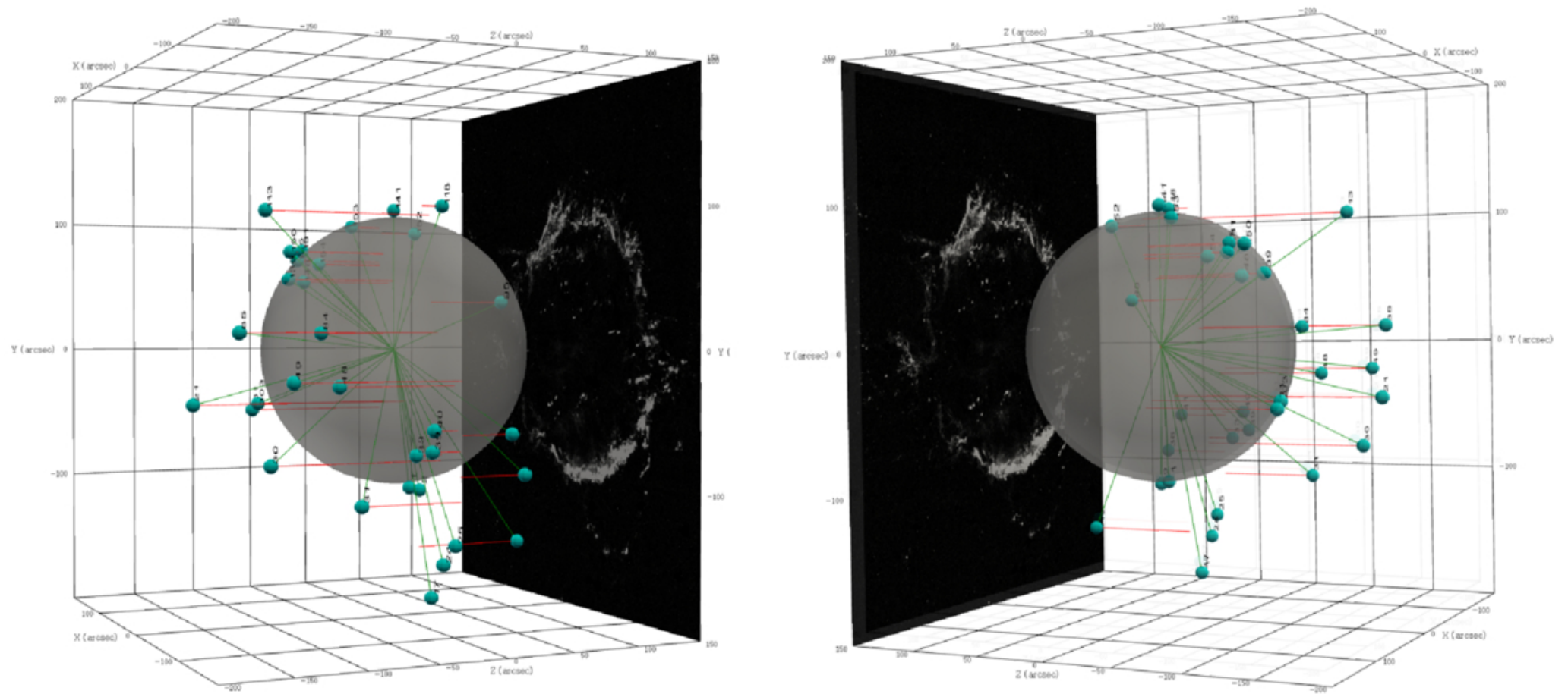
Figure 10. from Bon-Chul Koo et al 2025 Astrophys. J. Suppl. 280 doi:10.3847/1538-4365/adf0fd https://dx.doi.org/10.3847/1538-4365/adf0fd © 2025. The Author(s). Published by the American Astronomical Society.
