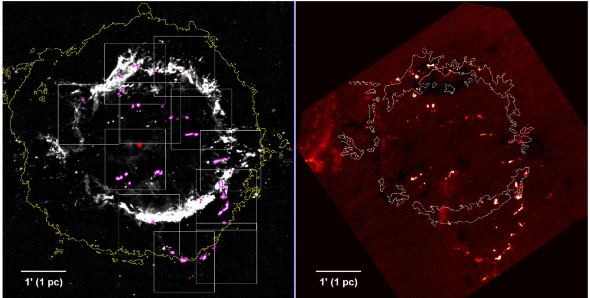
Figure 1. from Bon-Chul Koo et al 2025 Astrophys. J. Suppl. 280 doi:10.3847/1538-4365/adf0fd https://dx.doi.org/10.3847/1538-4365/adf0fd © 2025. The Author(s). Published by the American Astronomical Society.
