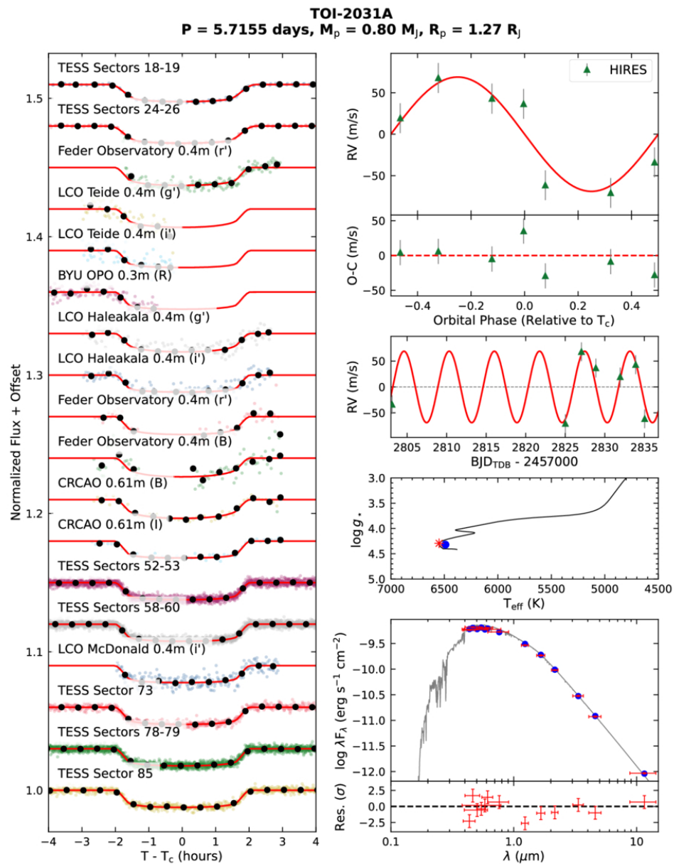
Figure 4. Data and EXOFASTv2 fit results from Samuel W. Yee et al 2025 Astrophys. J. Suppl. 280 doi:10.3847/1538-4365/aded0d https://dx.doi.org/10.3847/1538-4365/aded0d © 2025. The Author(s). Published by the American Astronomical Society.
