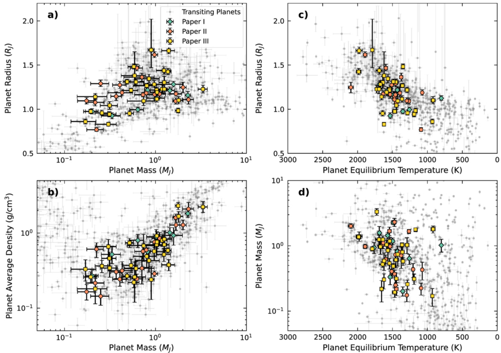
Figure 3. from Samuel W. Yee et al 2025 Astrophys. J. Suppl. 280 doi:10.3847/1538-4365/aded0d https://dx.doi.org/10.3847/1538-4365/aded0d © 2025. The Author(s). Published by the American Astronomical Society.
