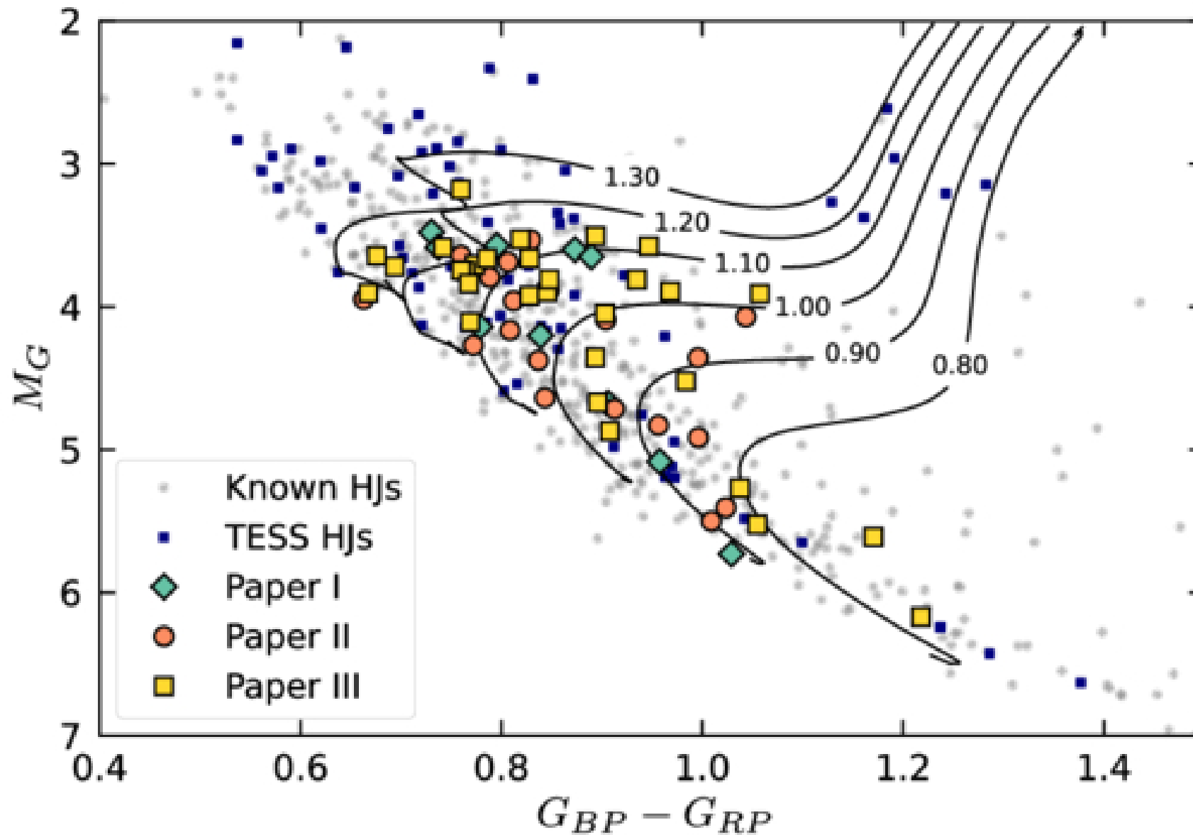
Figure 2. from Samuel W. Yee et al 2025 Astrophys. J. Suppl. 280 doi:10.3847/1538-4365/aded0d https://dx.doi.org/10.3847/1538-4365/aded0d © 2025. The Author(s). Published by the American Astronomical Society.
