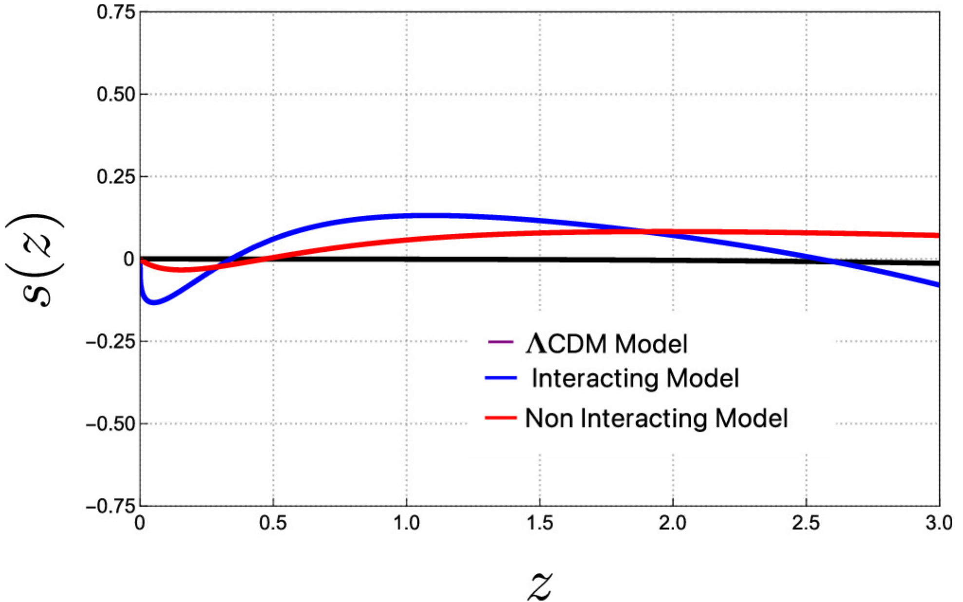
Figure 10. from Himanshu Chaudhary et al 2025 Astrophys. J. Suppl. 278 doi:10.3847/1538-4365/adc679 https://dx.doi.org/10.3847/1538-4365/adc679 © 2025. The Author(s). Published by the American Astronomical Society.
