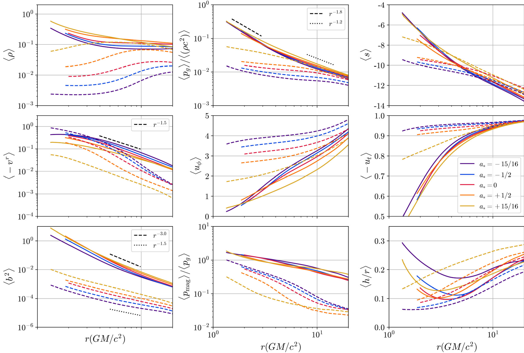
Figure 8. from Vedant Dhruv et al 2025 Astrophys. J. Suppl. 277 doi:10.3847/1538-4365/adaea6 https://dx.doi.org/10.3847/1538-4365/adaea6 © 2025. The Author(s). Published by the American Astronomical Society.
