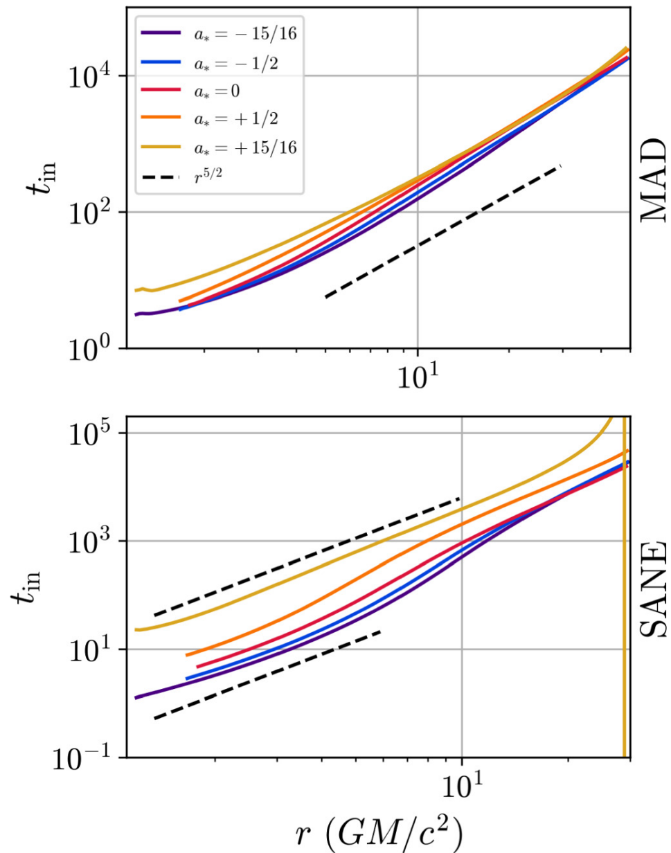
Figure 6. from Vedant Dhruv et al 2025 Astrophys. J. Suppl. 277 doi:10.3847/1538-4365/adaea6 https://dx.doi.org/10.3847/1538-4365/adaea6 © 2025. The Author(s). Published by the American Astronomical Society.
