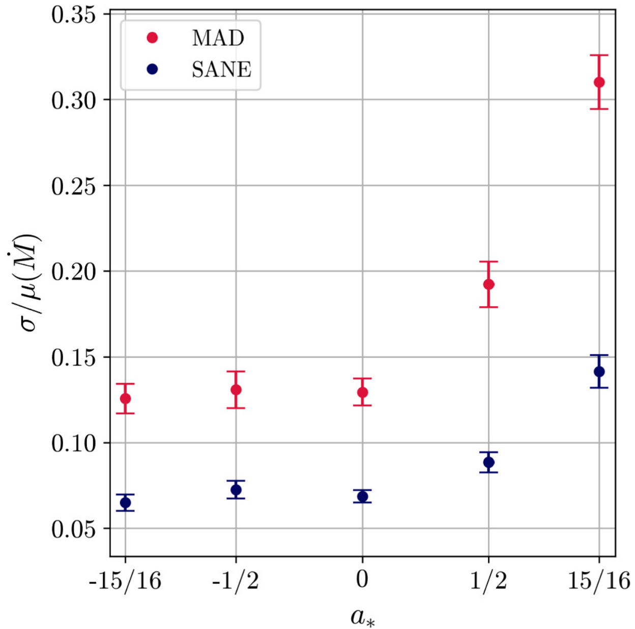
Figure 5. from Vedant Dhruv et al 2025 Astrophys. J. Suppl. 277 doi:10.3847/1538-4365/adaea6 https://dx.doi.org/10.3847/1538-4365/adaea6 © 2025. The Author(s). Published by the American Astronomical Society.
