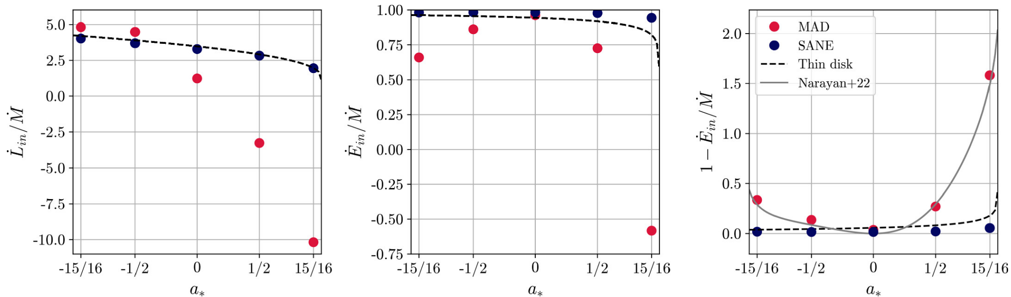
Figure 3. from Vedant Dhruv et al 2025 Astrophys. J. Suppl. 277 doi:10.3847/1538-4365/adaea6 https://dx.doi.org/10.3847/1538-4365/adaea6 © 2025. The Author(s). Published by the American Astronomical Society.
