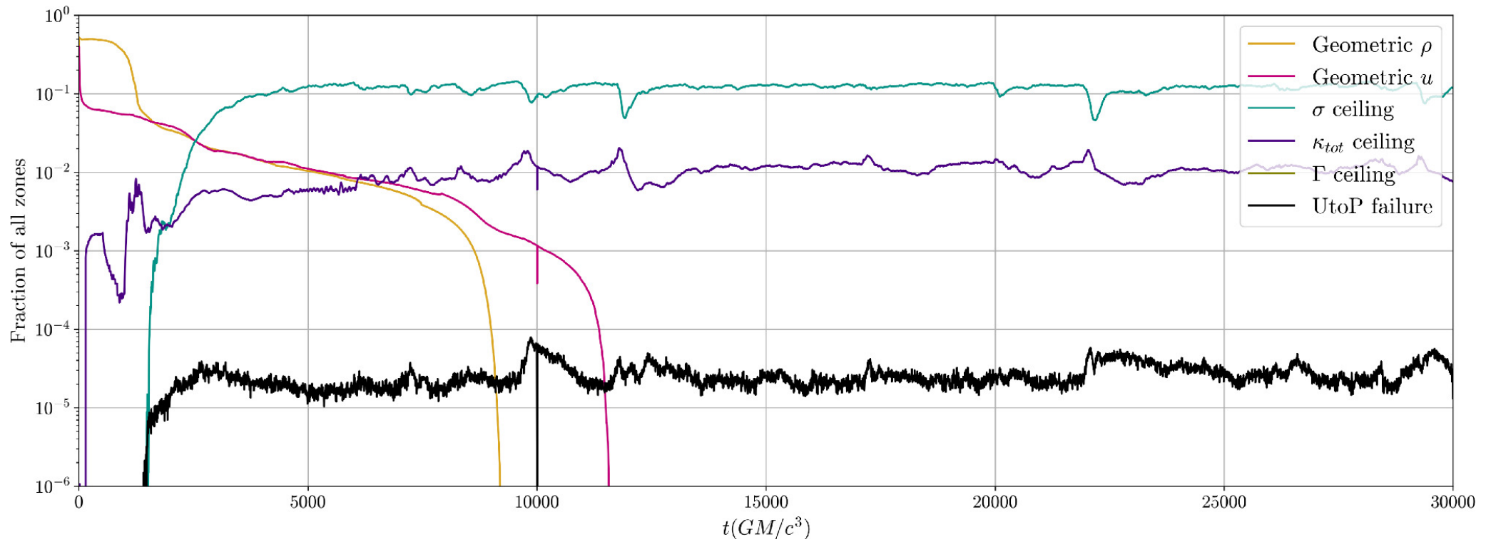
Figure 20. from Vedant Dhruv et al 2025 Astrophys. J. Suppl. 277 doi:10.3847/1538-4365/adaea6 https://dx.doi.org/10.3847/1538-4365/adaea6 © 2025. The Author(s). Published by the American Astronomical Society.
