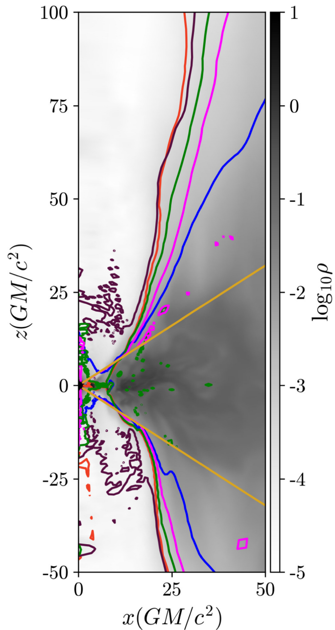
Figure 19. from Vedant Dhruv et al 2025 Astrophys. J. Suppl. 277 doi:10.3847/1538-4365/adaea6 https://dx.doi.org/10.3847/1538-4365/adaea6 © 2025. The Author(s). Published by the American Astronomical Society.
