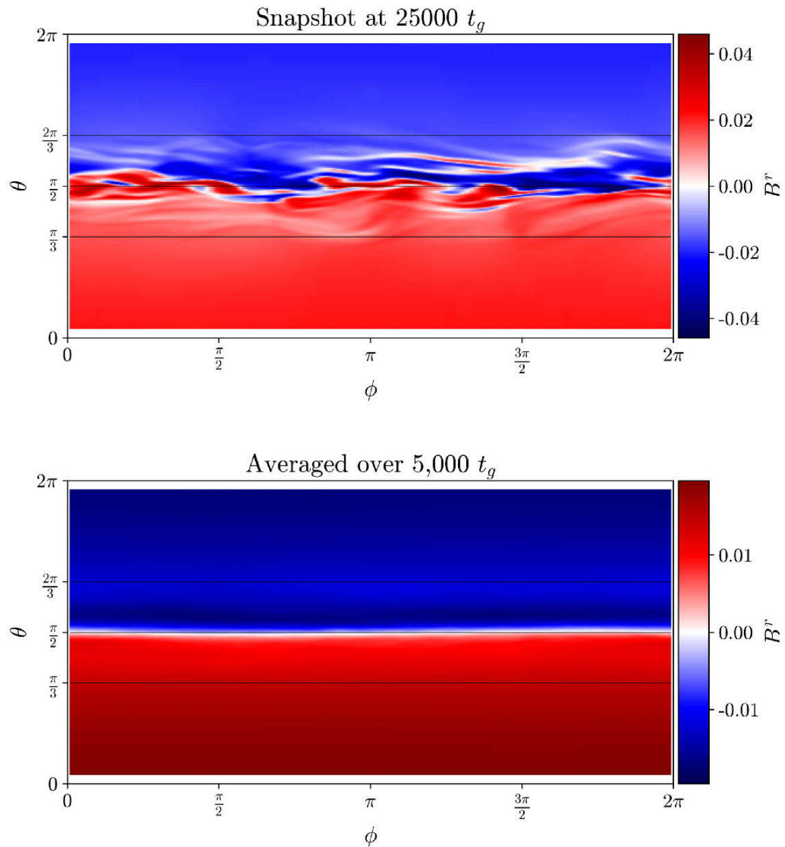
Figure 18. from Vedant Dhruv et al 2025 Astrophys. J. Suppl. 277 doi:10.3847/1538-4365/adaea6 https://dx.doi.org/10.3847/1538-4365/adaea6 © 2025. The Author(s). Published by the American Astronomical Society.
