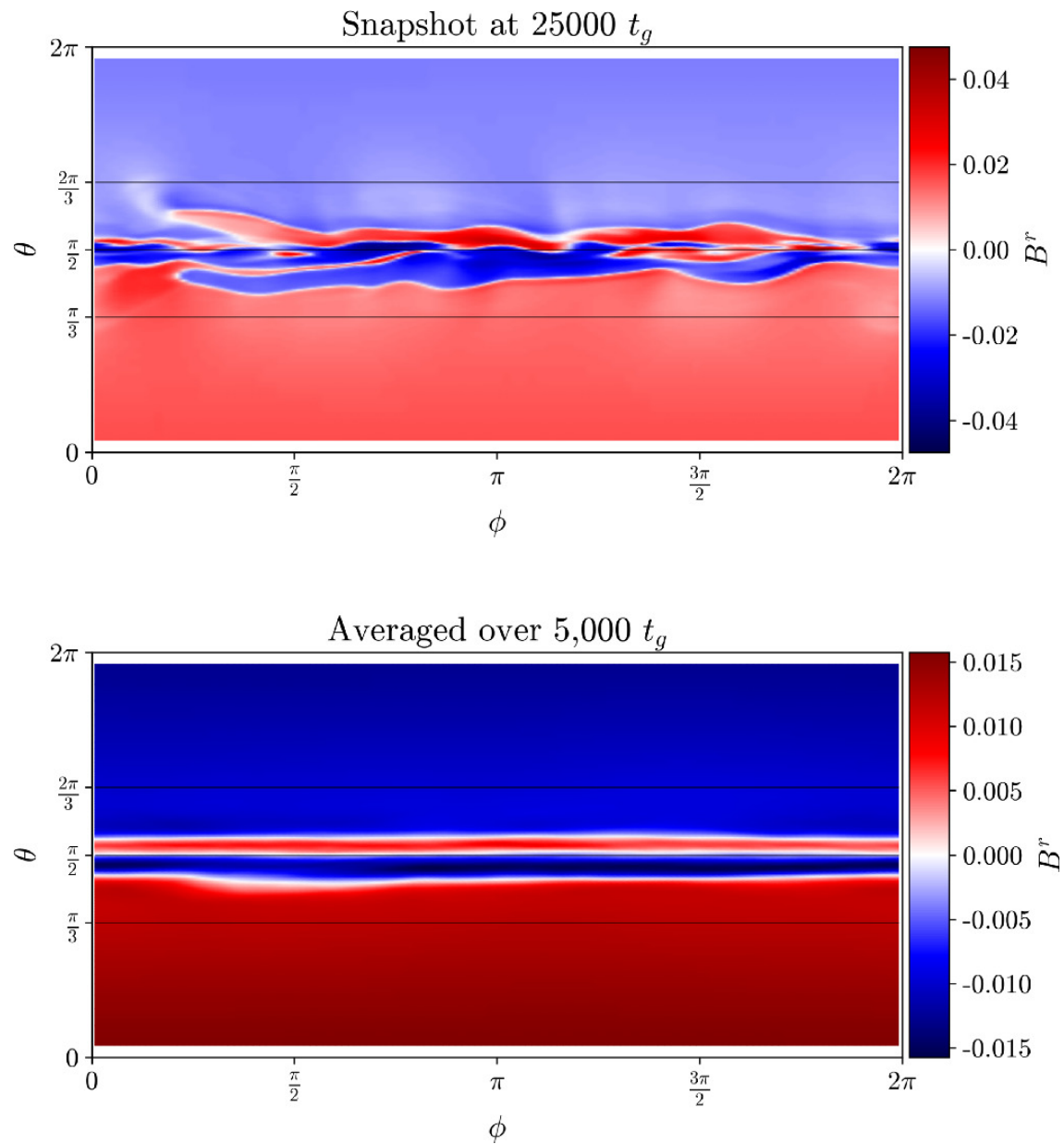
Figure 17. from Vedant Dhruv et al 2025 Astrophys. J. Suppl. 277 doi:10.3847/1538-4365/adaea6 https://dx.doi.org/10.3847/1538-4365/adaea6 © 2025. The Author(s). Published by the American Astronomical Society.
