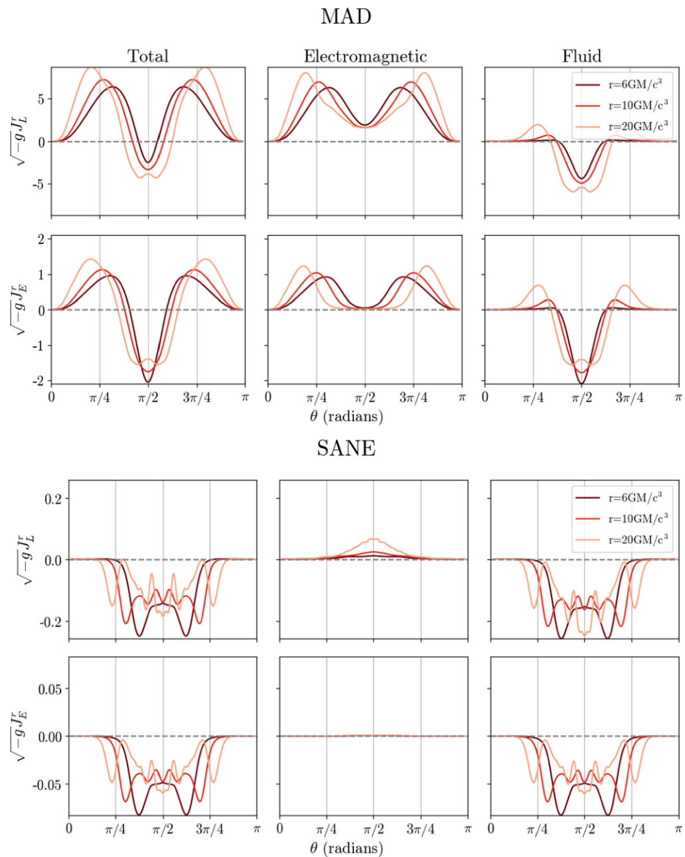
Figure 12. from Vedant Dhruv et al 2025 Astrophys. J. Suppl. 277 doi:10.3847/1538-4365/adaea6 https://dx.doi.org/10.3847/1538-4365/adaea6 © 2025. The Author(s). Published by the American Astronomical Society.
