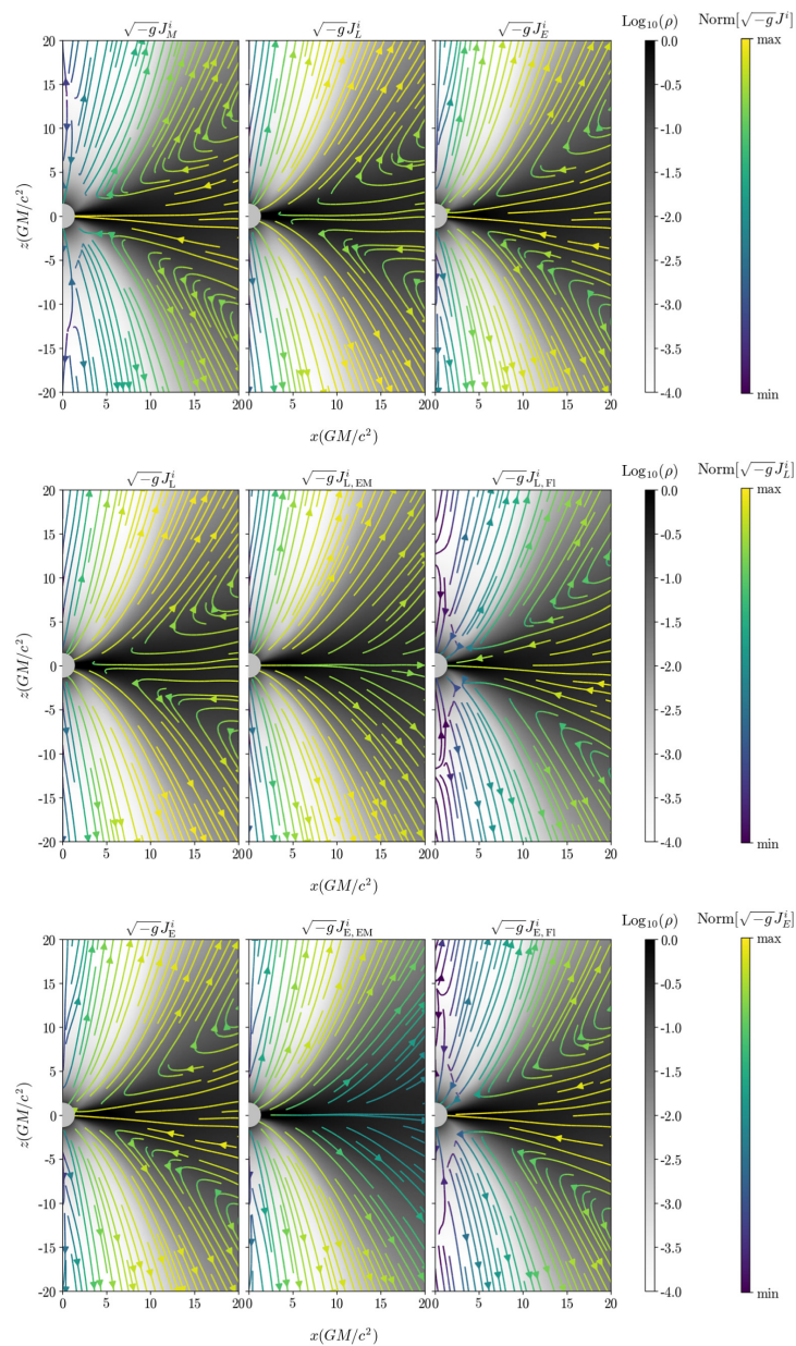
Figure 11. from Vedant Dhruv et al 2025 Astrophys. J. Suppl. 277 doi:10.3847/1538-4365/adaea6 https://dx.doi.org/10.3847/1538-4365/adaea6 © 2025. The Author(s). Published by the American Astronomical Society.
