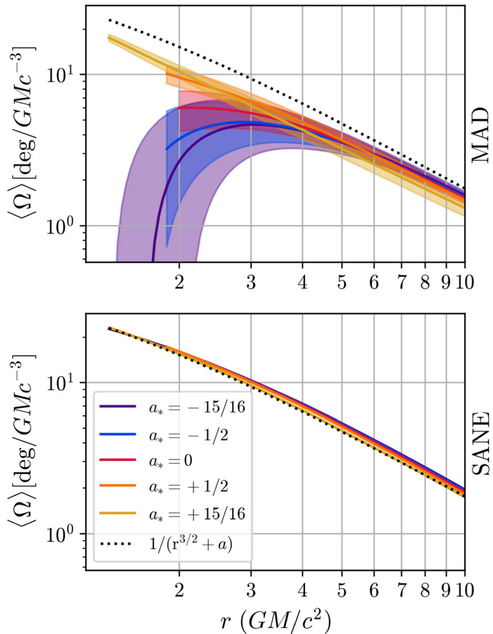
Figure 10. from Vedant Dhruv et al 2025 Astrophys. J. Suppl. 277 doi:10.3847/1538-4365/adaea6 https://dx.doi.org/10.3847/1538-4365/adaea6 © 2025. The Author(s). Published by the American Astronomical Society.
