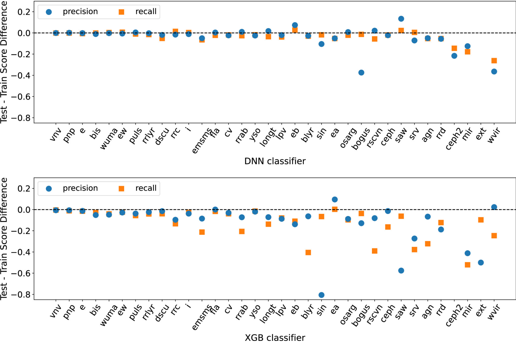
Figure 9. from Brian F. Healy et al 2024 Astrophys. J. Suppl. 272 doi:10.3847/1538-4365/ad33c6 https://dx.doi.org/10.3847/1538-4365/ad33c6 © 2024. The Author(s). Published by the American Astronomical Society.
