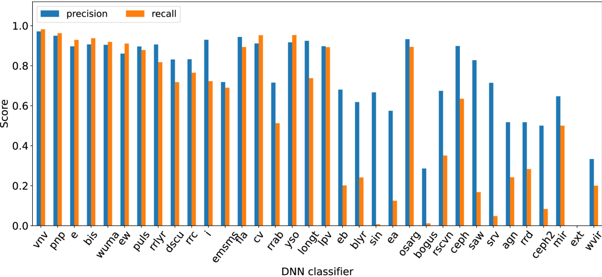
Figure 7. from Brian F. Healy et al 2024 Astrophys. J. Suppl. 272 doi:10.3847/1538-4365/ad33c6 https://dx.doi.org/10.3847/1538-4365/ad33c6 © 2024. The Author(s). Published by the American Astronomical Society.
