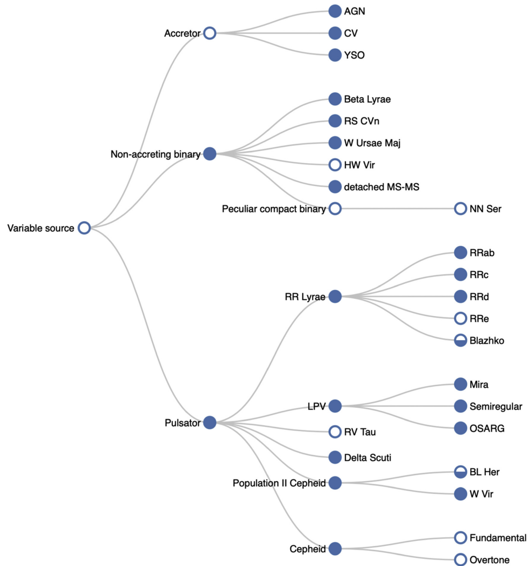
Figure 2. from Brian F. Healy et al 2024 Astrophys. J. Suppl. 272 doi:10.3847/1538-4365/ad33c6 https://dx.doi.org/10.3847/1538-4365/ad33c6 © 2024. The Author(s). Published by the American Astronomical Society.
