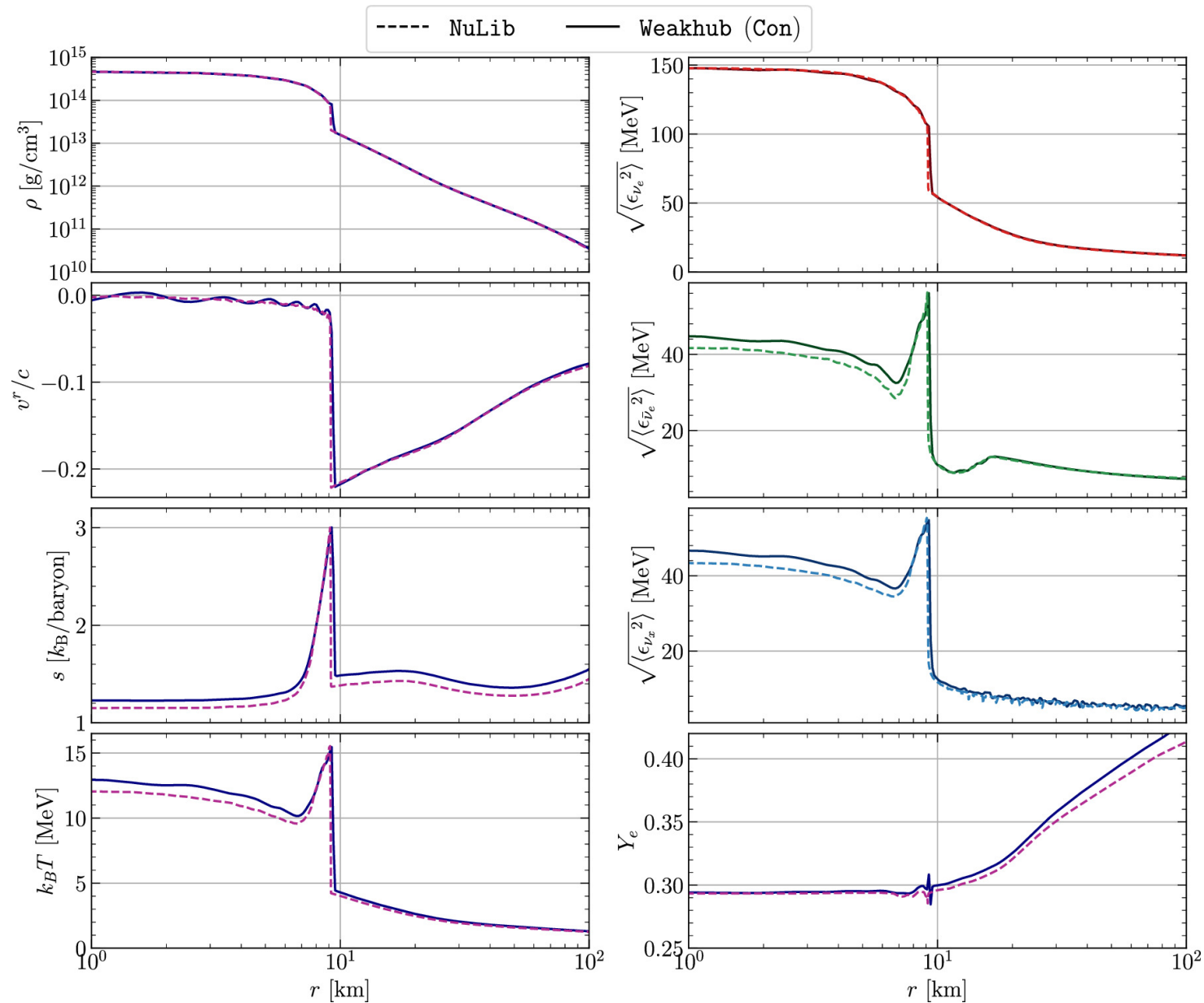
Figure 5. from Harry Ho-Yin Ng et al 2024 Astrophys. J. Suppl. 272 doi:10.3847/1538-4365/ad2fbd https://dx.doi.org/10.3847/1538-4365/ad2fbd © 2024. The Author(s). Published by the American Astronomical Society.
