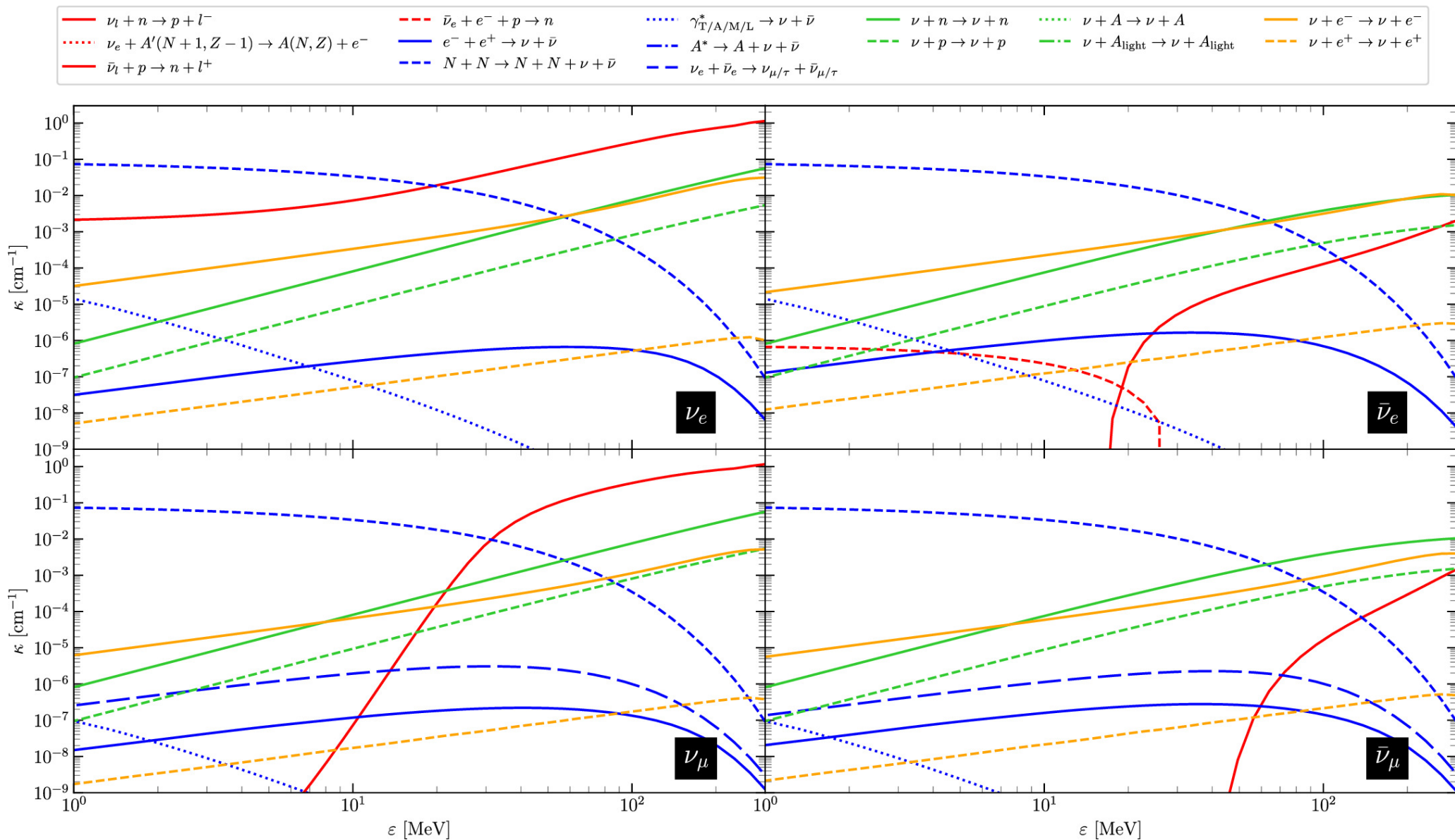
Figure 3. from Harry Ho-Yin Ng et al 2024 Astrophys. J. Suppl. 272 doi:10.3847/1538-4365/ad2fbd https://dx.doi.org/10.3847/1538-4365/ad2fbd © 2024. The Author(s). Published by the American Astronomical Society.
