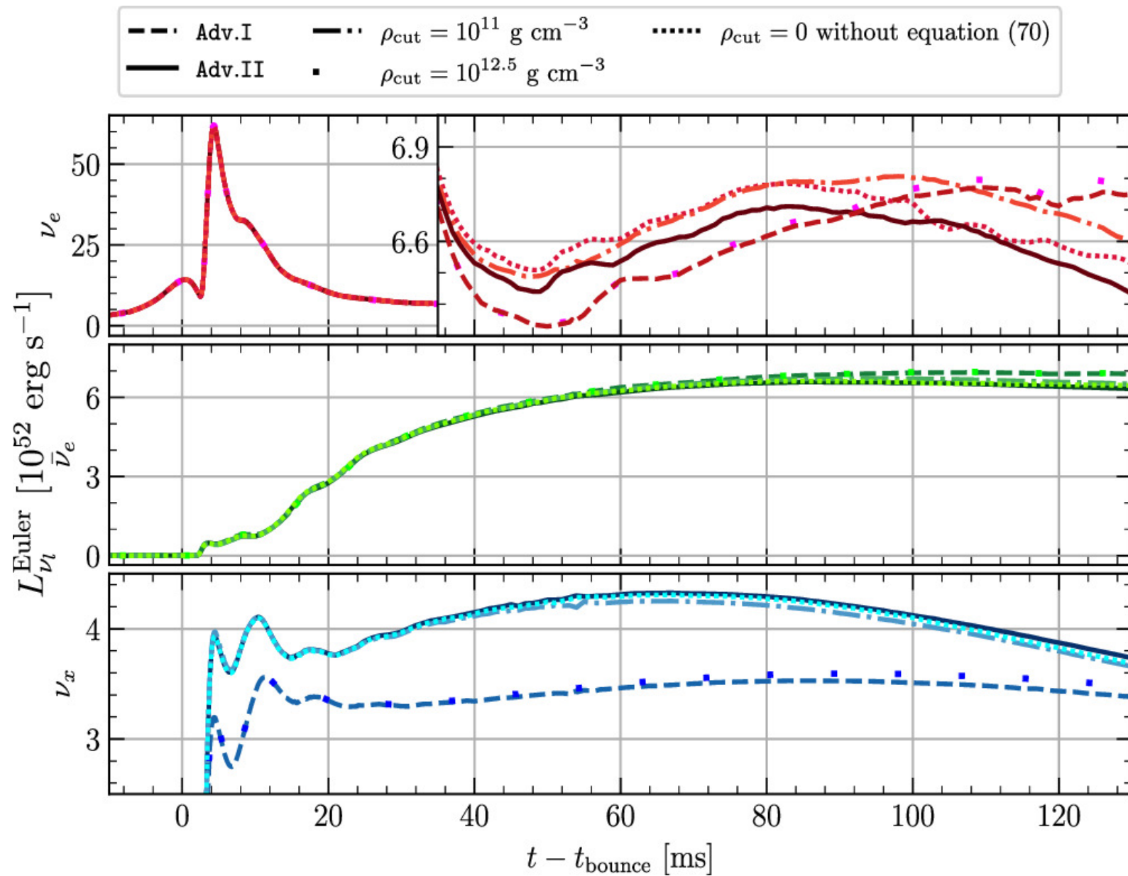
Figure 10. from Harry Ho-Yin Ng et al 2024 Astrophys. J. Suppl. 272 doi:10.3847/1538-4365/ad2fbd https://dx.doi.org/10.3847/1538-4365/ad2fbd © 2024. The Author(s). Published by the American Astronomical Society.
