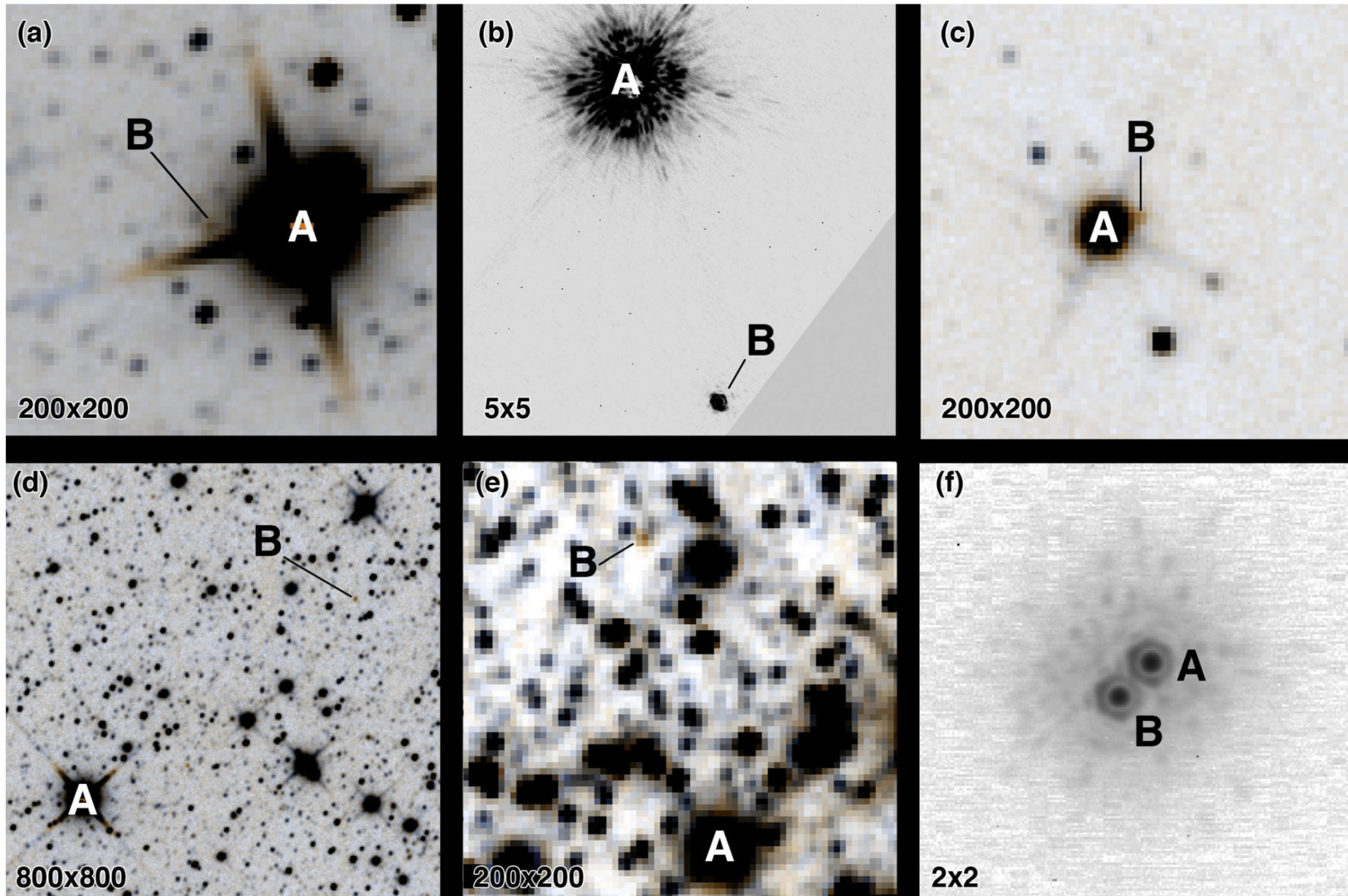
Figure 1. from J. Davy Kirkpatrick et al 2024 Astrophys. J. Suppl. 271 doi:10.3847/1538-4365/ad24e2 https://dx.doi.org/10.3847/1538-4365/ad24e2 © 2024. The Author(s). Published by the American Astronomical Society.
