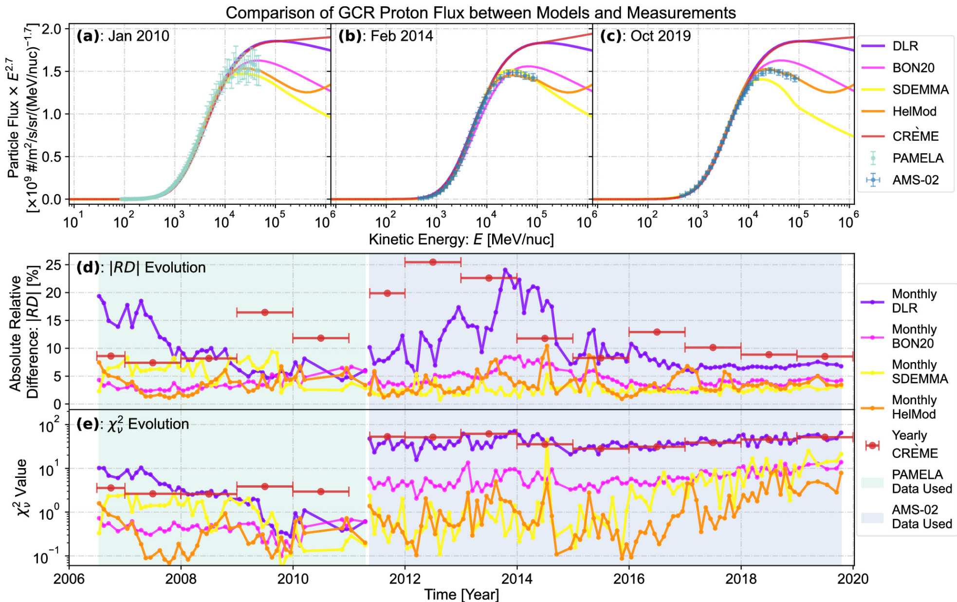
Figure 8. from Weihao Liu et al 2024 Astrophys. J. Suppl. 271 doi:10.3847/1538-4365/ad18ad https://dx.doi.org/10.3847/1538-4365/ad18ad © 2024. The Author(s). Published by the American Astronomical Society.
