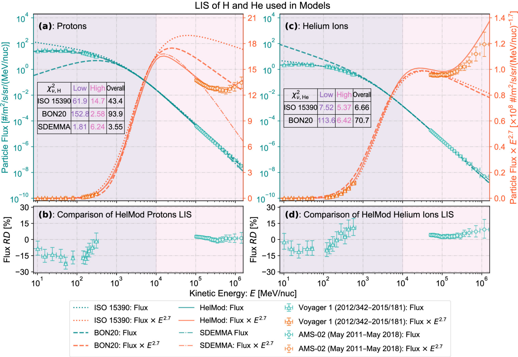
Figure 6. from Weihao Liu et al 2024 Astrophys. J. Suppl. 271 doi:10.3847/1538-4365/ad18ad https://dx.doi.org/10.3847/1538-4365/ad18ad © 2024. The Author(s). Published by the American Astronomical Society.
