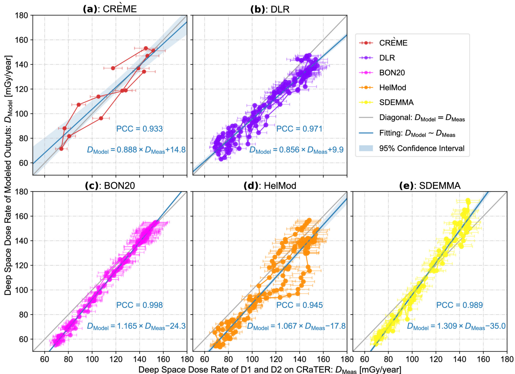
Figure 4. from Weihao Liu et al 2024 Astrophys. J. Suppl. 271 doi:10.3847/1538-4365/ad18ad https://dx.doi.org/10.3847/1538-4365/ad18ad © 2024. The Author(s). Published by the American Astronomical Society.
