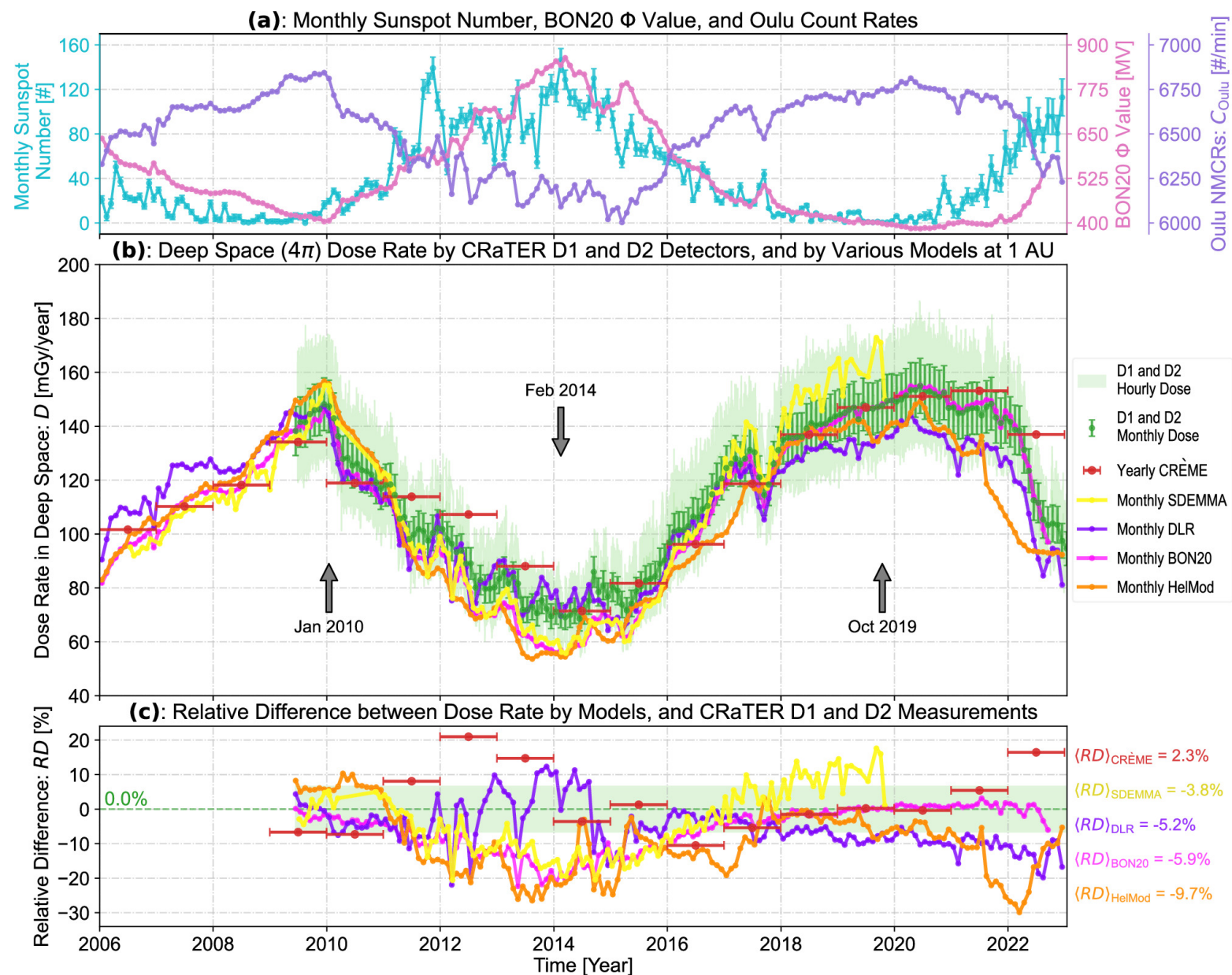
Figure 3. from Weihaio Liu et al 2024 Astrophys. J. Suppl. 271 doi:10.3847/1538-4365/ad18ad https://dx.doi.org/10.3847/1538-4365/ad18ad © 2024. The Author(s). Published by the American Astronomical Society.
