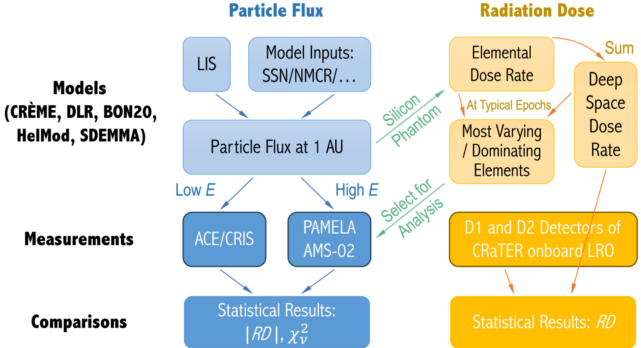
Figure 2. from Weihao Liu et al 2024 Astrophys. J. Suppl. 271 doi:10.3847/1538-4365/ad18ad https://dx.doi.org/10.3847/1538-4365/ad18ad © 2024. The Author(s). Published by the American Astronomical Society.
