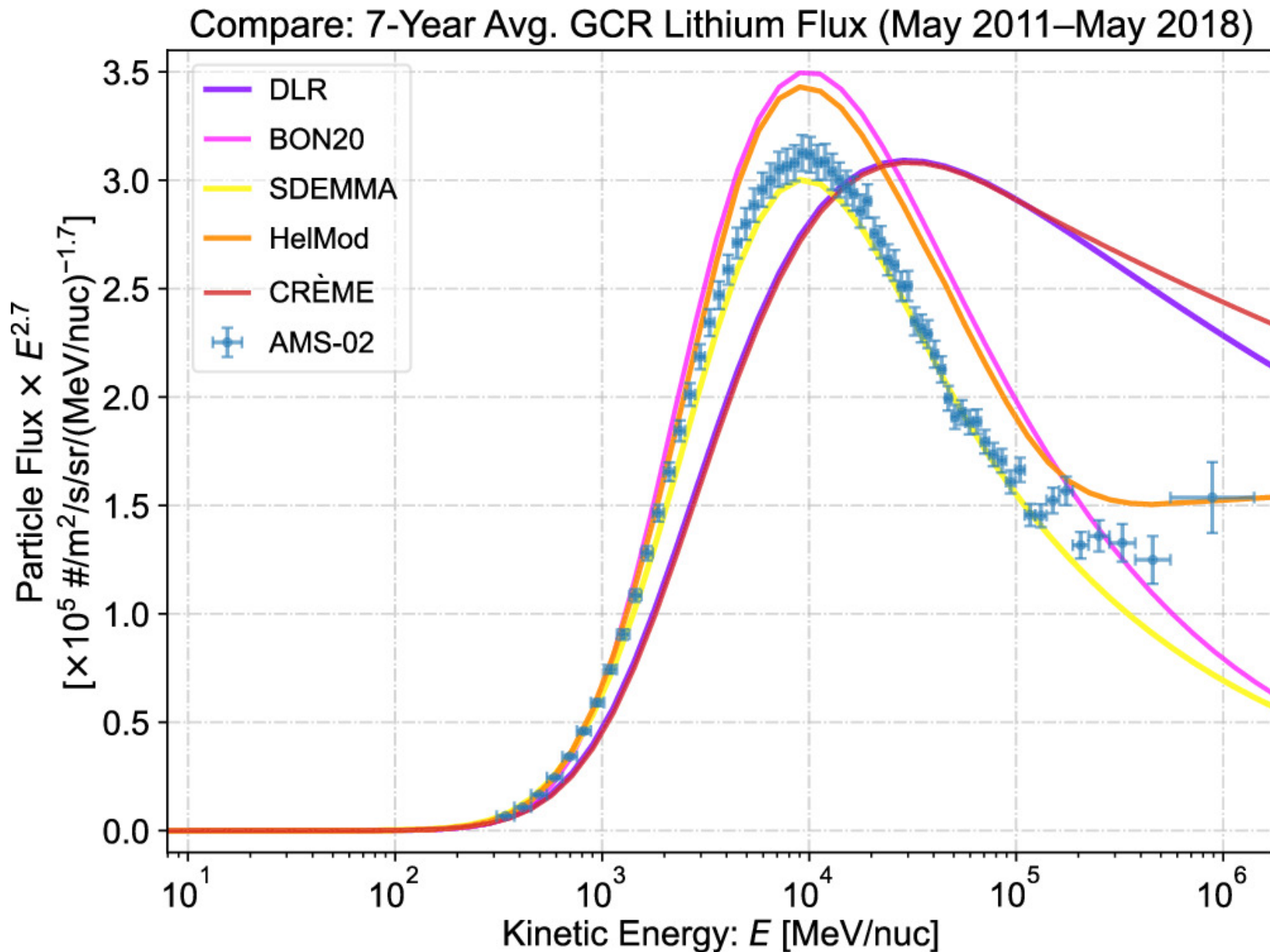
Figure 16. from Weihao Liu et al 2024 Astrophys. J. Suppl. 271 doi:10.3847/1538-4365/ad18ad https://dx.doi.org/10.3847/1538-4365/ad18ad © 2024. The Author(s). Published by the American Astronomical Society.
