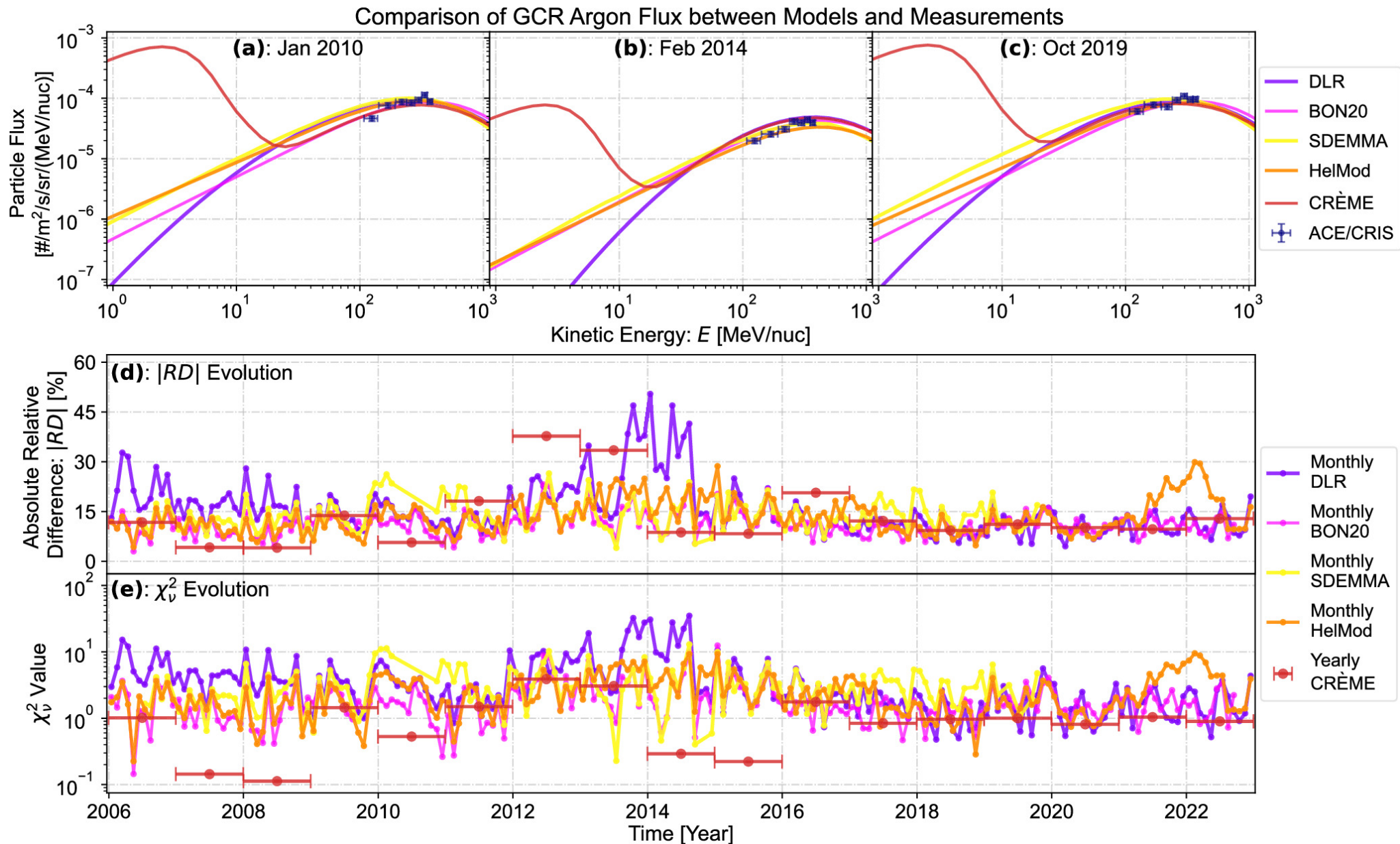
Figure 15. from Weihao Liu et al 2024 Astrophys. J. Suppl. 271 doi:10.3847/1538-4365/ad18ad https://dx.doi.org/10.3847/1538-4365/ad18ad © 2024. The Author(s). Published by the American Astronomical Society.
