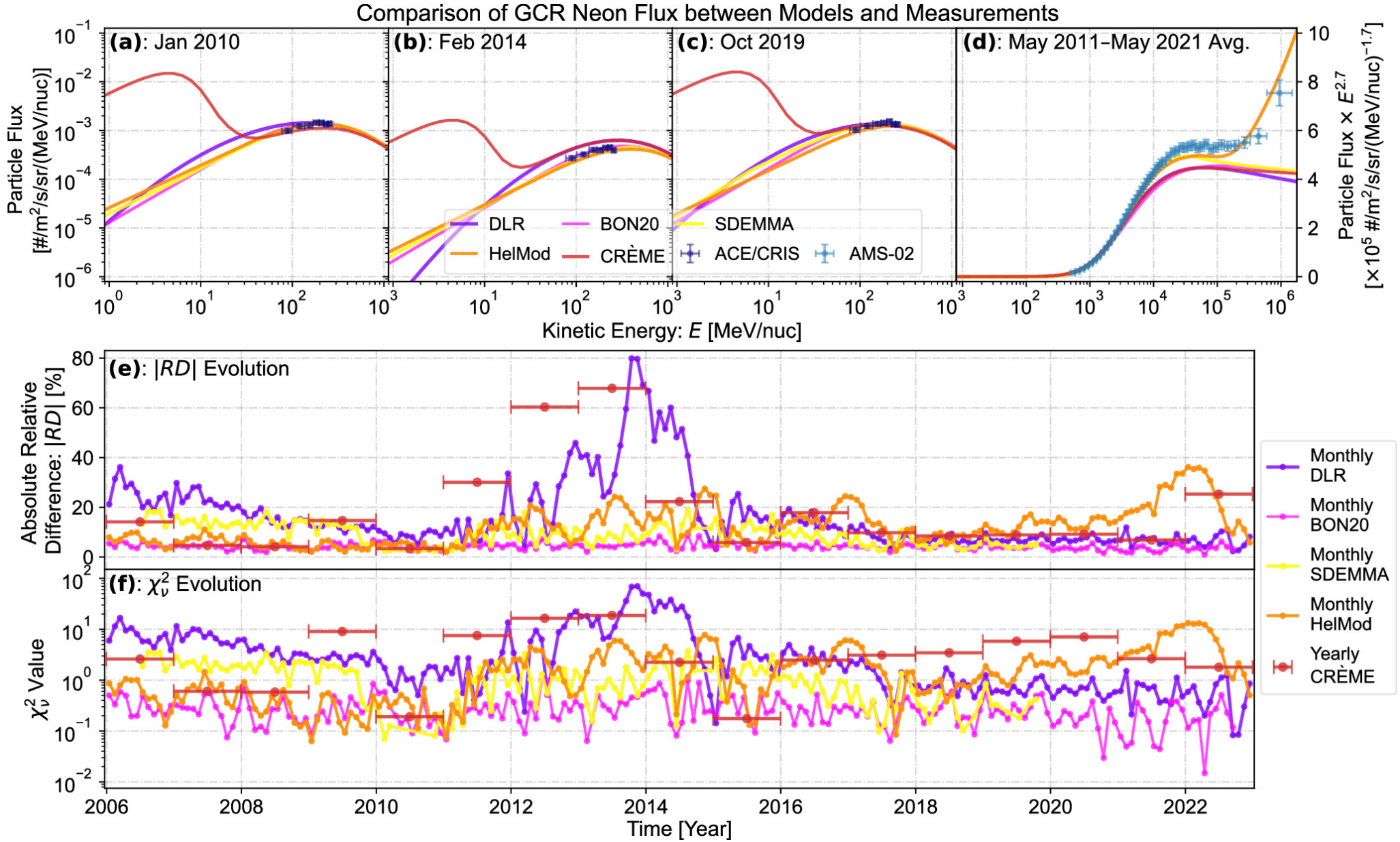
Figure 14. from Weihao Liu et al 2024 Astrophys. J. Suppl. 271 doi:10.3847/1538-4365/ad18ad https://dx.doi.org/10.3847/1538-4365/ad18ad © 2024. The Author(s). Published by the American Astronomical Society.
