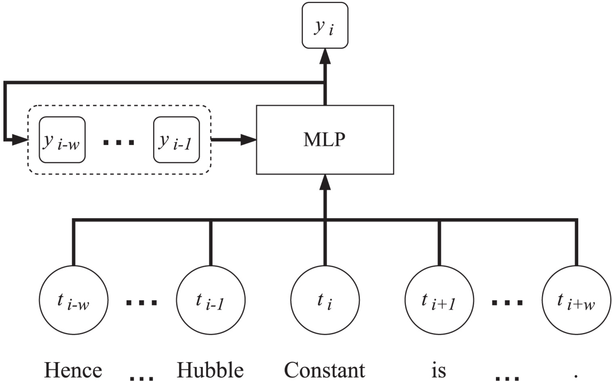
Figure 2. from Tom Crossland et al 2023 Astrophys. J. Suppl. 269 doi:10.3847/1538-4365/acf76a https://dx.doi.org/10.3847/1538-4365/acf76a © 2023. The Author(s). Published by the American Astronomical Society.
