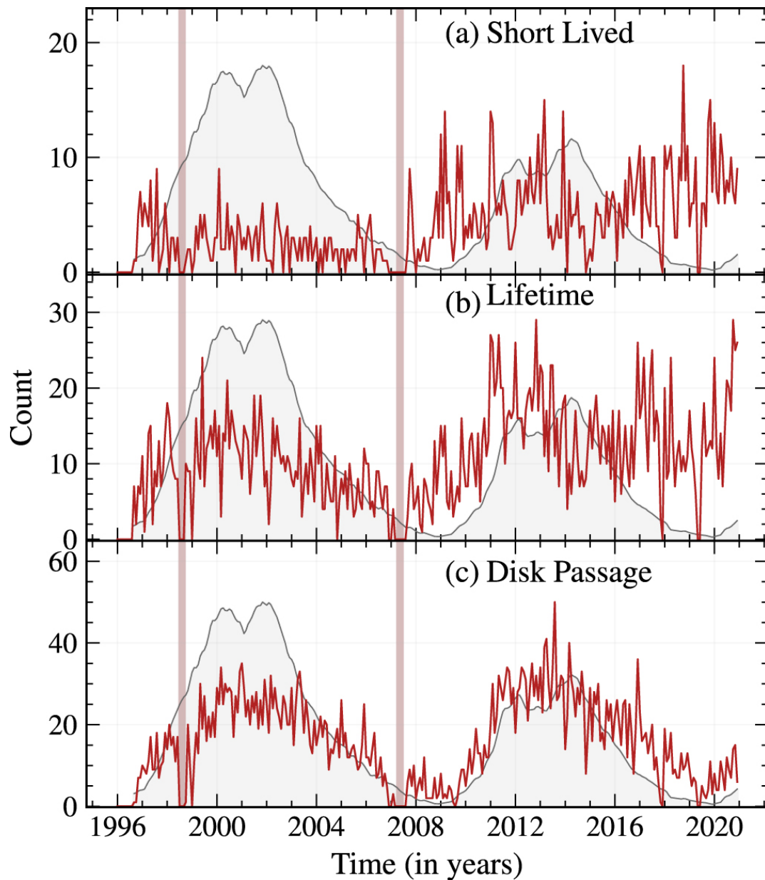
Figure 6. from Anu Sreedevi et al 2023 Astrophys. J. Suppl. 268 doi:10.3847/1538-4365/acec47 https://dx.doi.org/10.3847/1538-4365/acec47 © 2023. The Author(s). Published by the American Astronomical Society.
