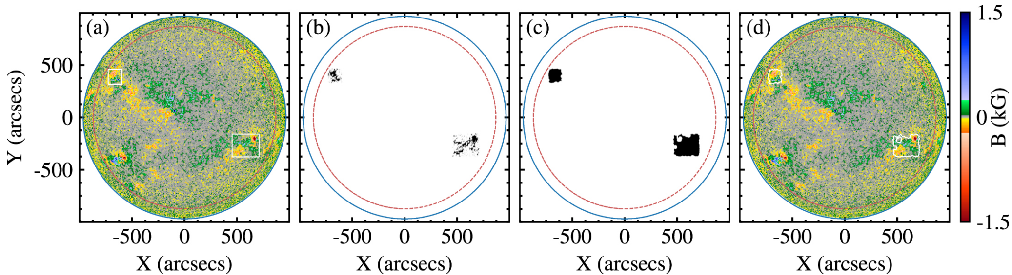
Figure 1. from Anu Sreedevi et al 2023 Astrophys. J. Suppl. 268 doi:10.3847/1538-4365/acec47 https://dx.doi.org/10.3847/1538-4365/acec47 © 2023. The Author(s). Published by the American Astronomical Society.
