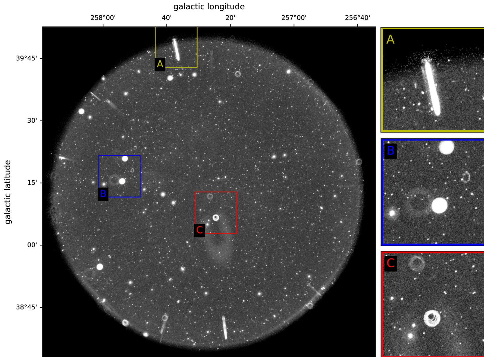
Figure 9. from Chase C. Million et al 2023 Astrophys. J. Suppl. 268 doi:10.3847/1538-4365/ace717 https://dx.doi.org/10.3847/1538-4365/ace717 © 2023. The Author(s). Published by the American Astronomical Society.
