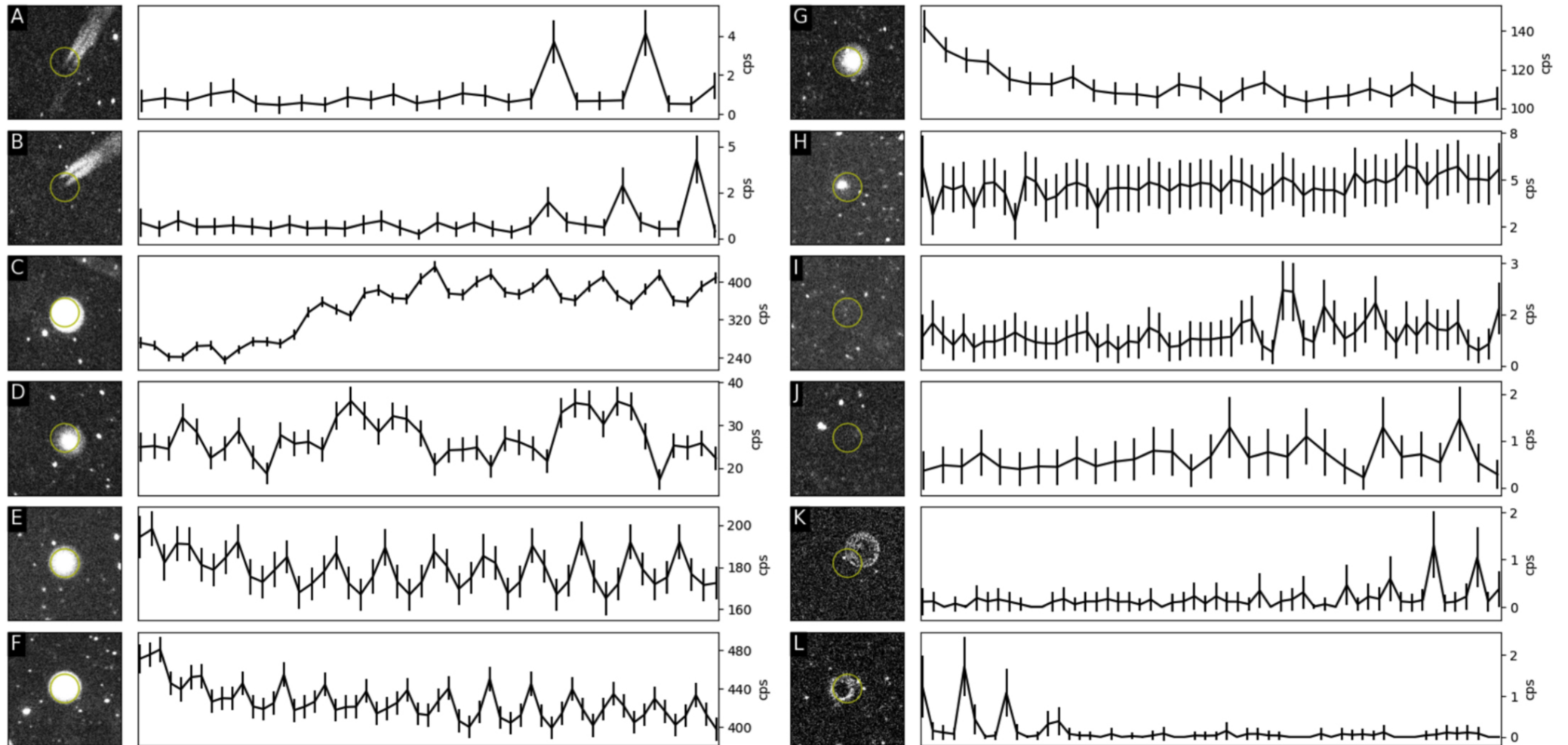
Figure 8. from Chase C. Million et al 2023 Astrophys. J. Suppl. 268 doi:10.3847/1538-4365/ace717 https://dx.doi.org/10.3847/1538-4365/ace717 © 2023. The Author(s). Published by the American Astronomical Society.
