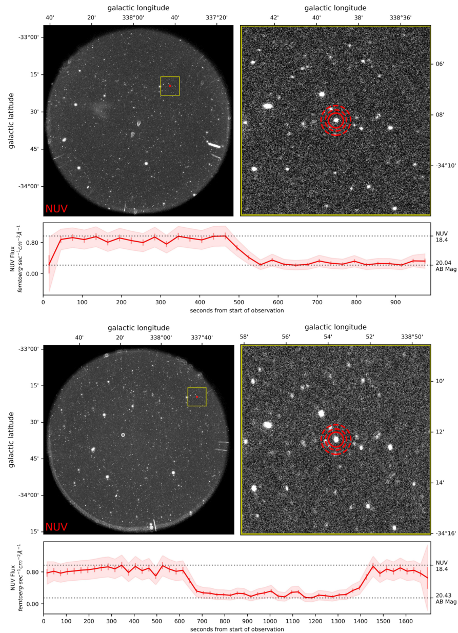
Figure 6. from Chase C. Million et al 2023 Astrophys. J. Suppl. 268 doi:10.3847/1538-4365/ace717 https://dx.doi.org/10.3847/1538-4365/ace717 © 2023. The Author(s). Published by the American Astronomical Society.
