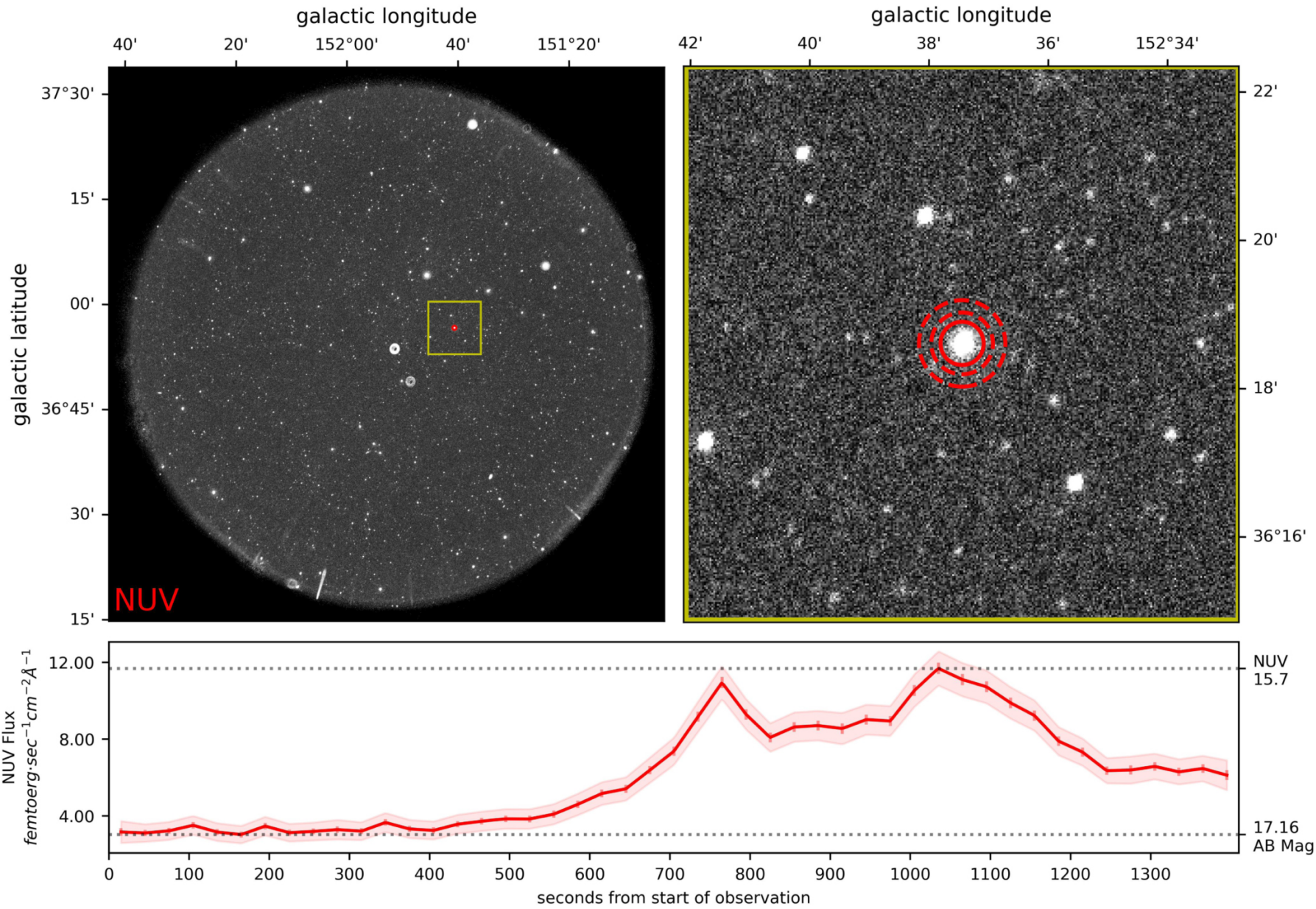
Figure 5. from Chase C. Million et al 2023 Astrophys. J. Suppl. 268 doi:10.3847/1538-4365/ace717 https://dx.doi.org/10.3847/1538-4365/ace717 © 2023. The Author(s). Published by the American Astronomical Society.
