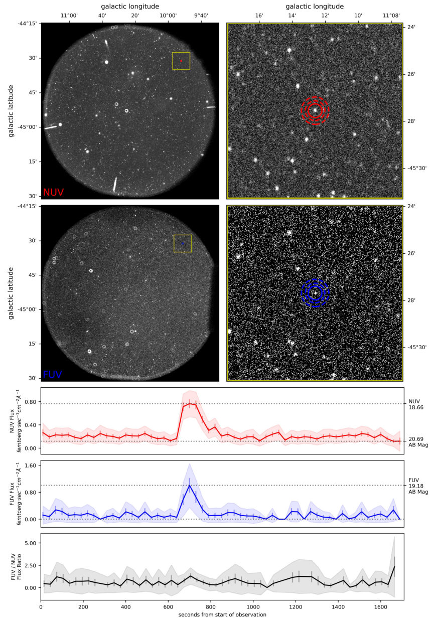
Figure 4. from Chase C. Million et al 2023 Astrophys. J. Suppl. 268 doi:10.3847/1538-4365/ace717 https://dx.doi.org/10.3847/1538-4365/ace717 © 2023. The Author(s). Published by the American Astronomical Society.
