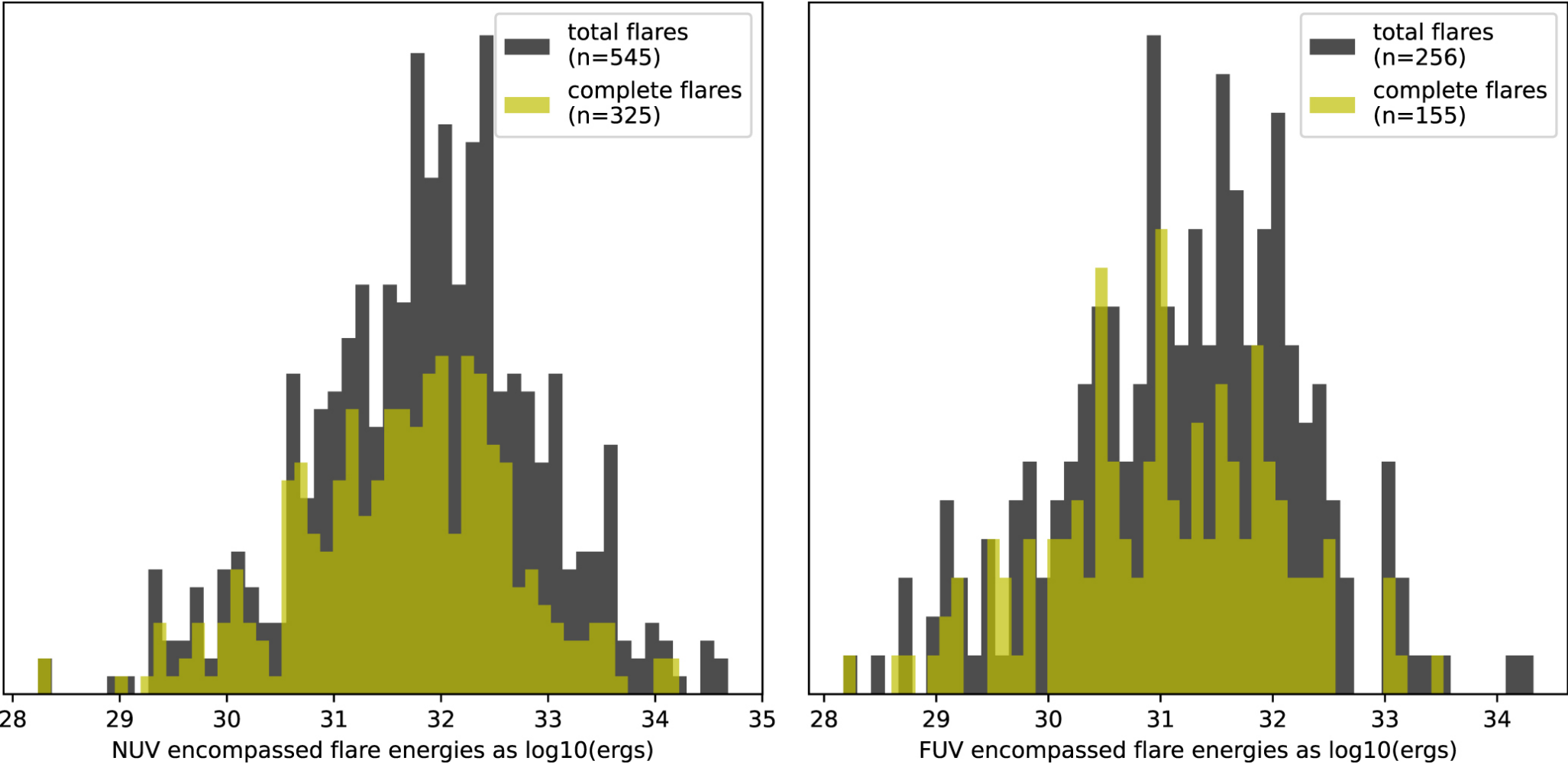
Figure 3. from Chase C. Million et al 2023 Astrophys. J. Suppl. 268 doi:10.3847/1538-4365/ace717 https://dx.doi.org/10.3847/1538-4365/ace717 © 2023. The Author(s). Published by the American Astronomical Society.
