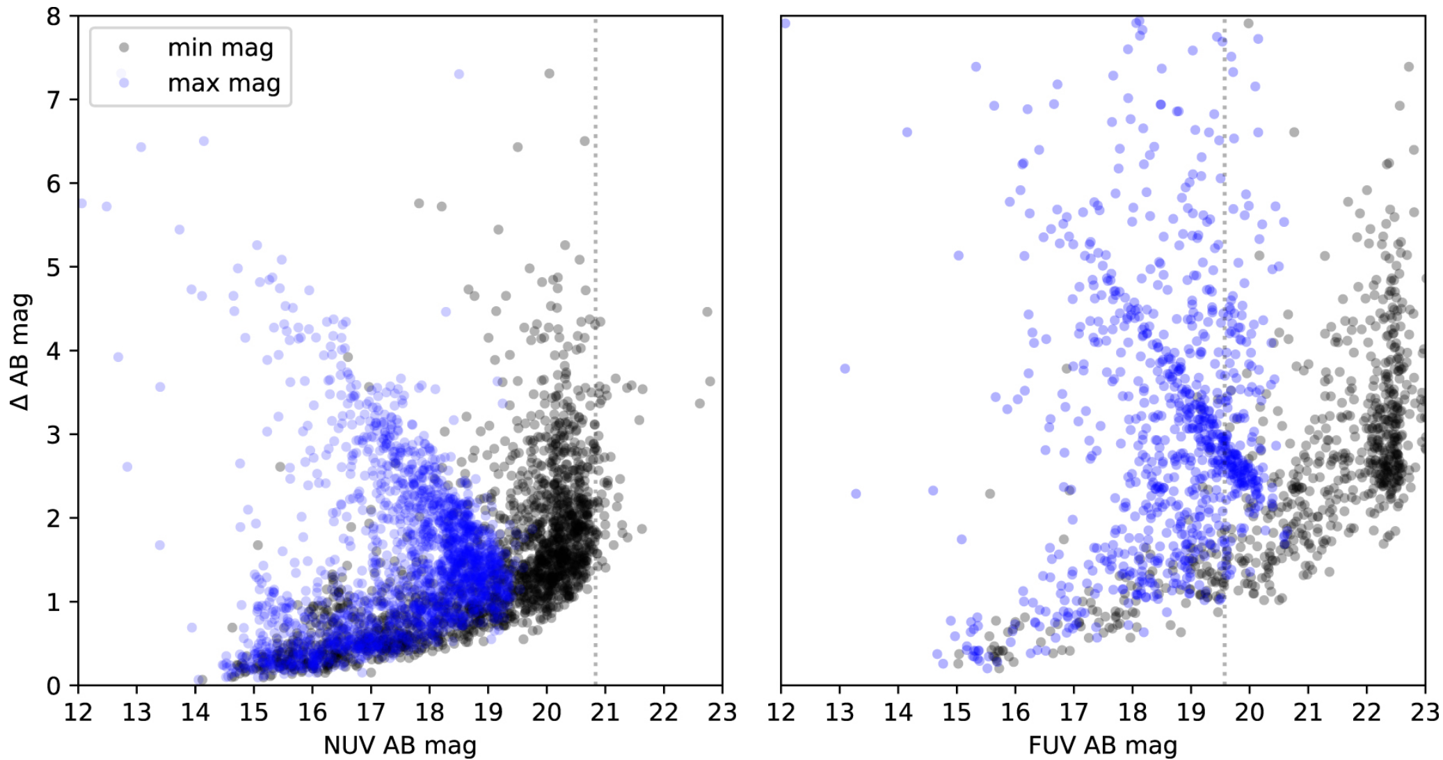
Figure 2. from Chase C. Million et al 2023 Astrophys. J. Suppl. 268 doi:10.3847/1538-4365/ace717 https://dx.doi.org/10.3847/1538-4365/ace717 © 2023. The Author(s). Published by the American Astronomical Society.
