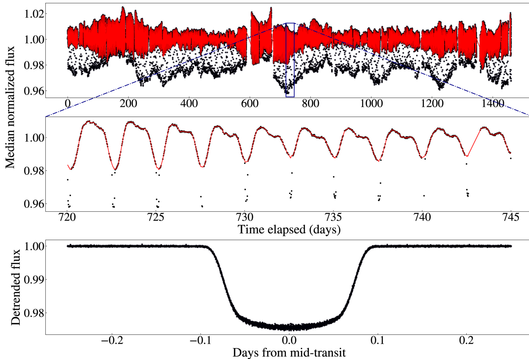
Figure 6. from Caleb I. Cañas et al 2023 Astrophys. J. Suppl. 265 doi:10.3847/1538-4365/acbcbe https://dx.doi.org/10.3847/1538-4365/acbcbe © 2023. The Author(s). Published by the American Astronomical Society.
