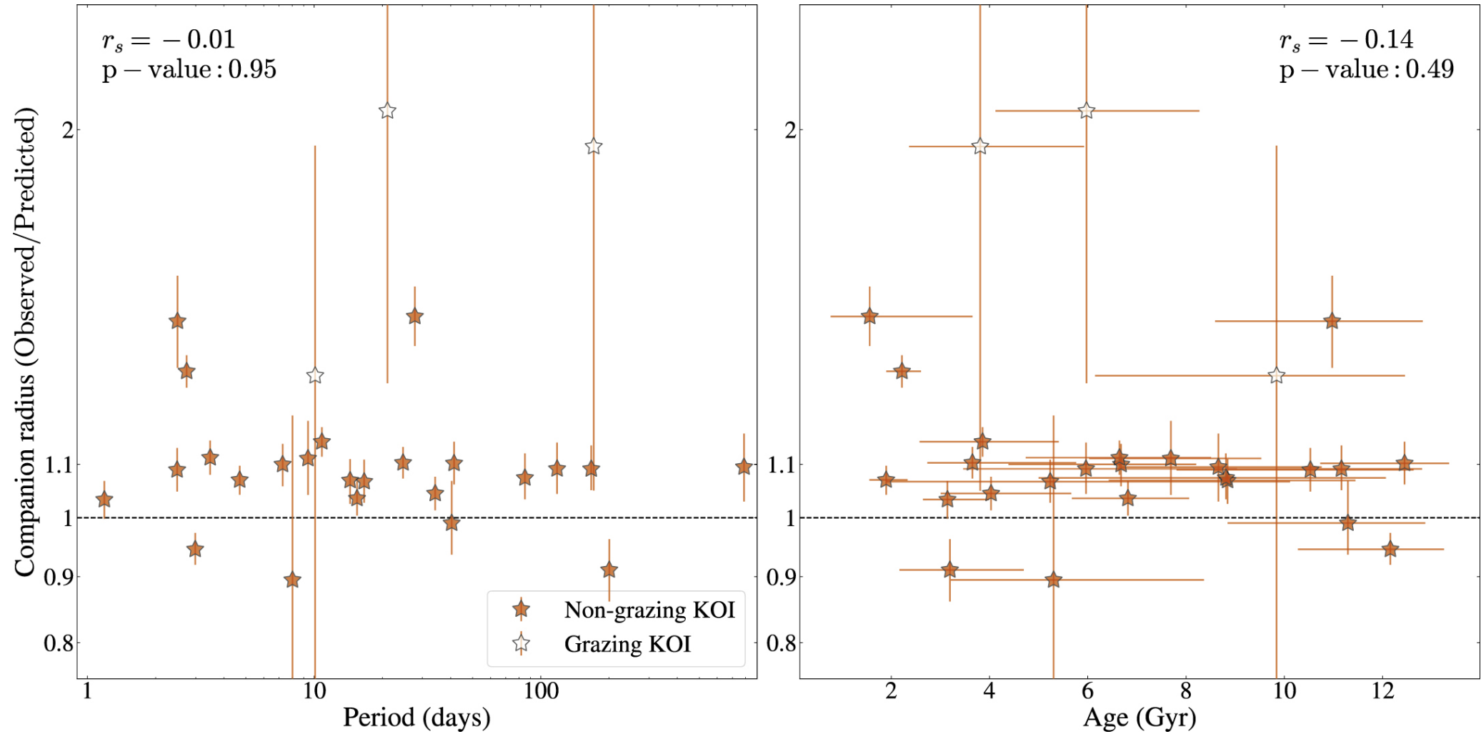
Figure 4. from Caleb I. Cañas et al 2023 Astrophys. J. Suppl. 265 doi:10.3847/1538-4365/acbcbe https://dx.doi.org/10.3847/1538-4365/acbcbe © 2023. The Author(s). Published by the American Astronomical Society.
