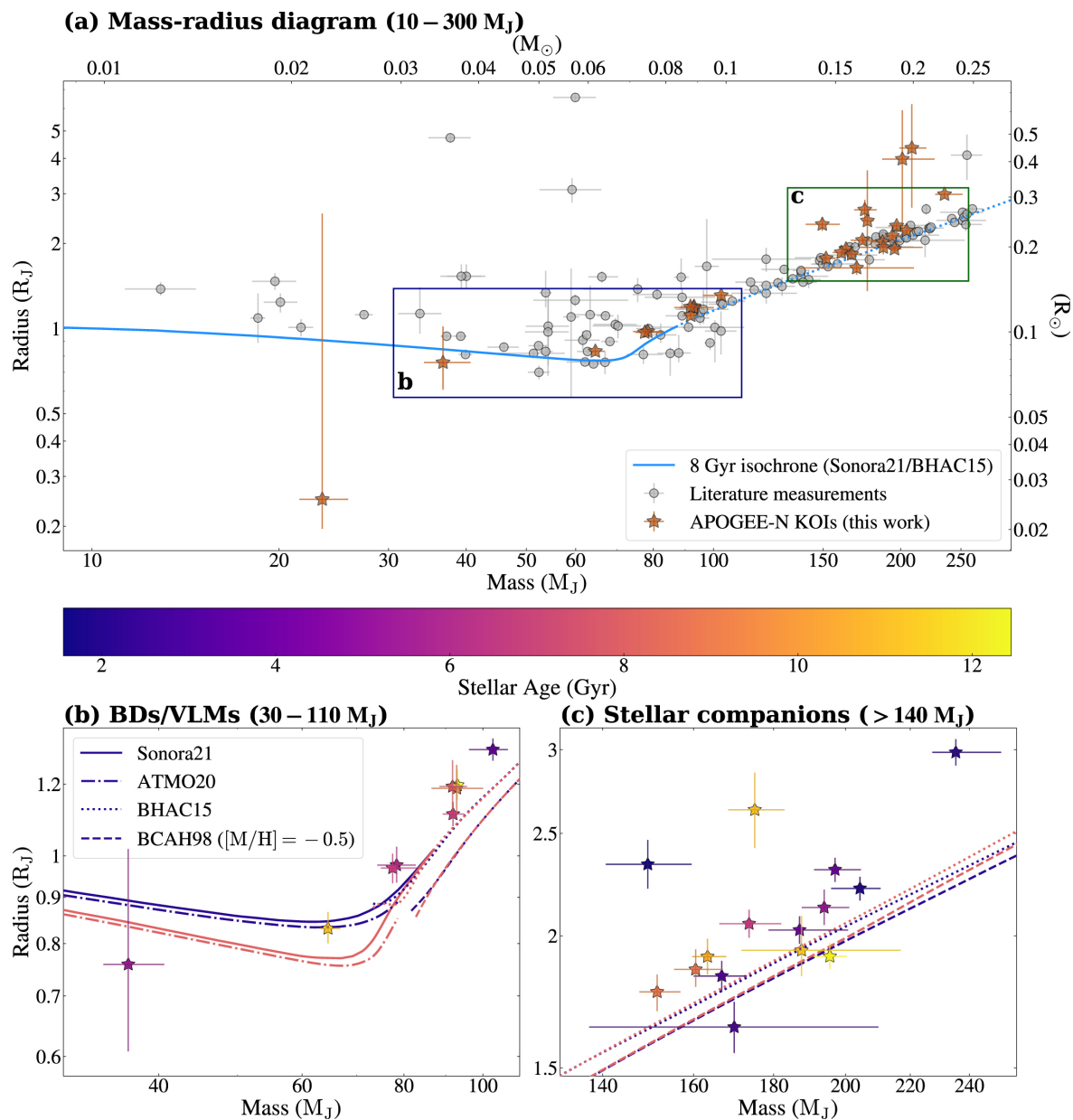
Figure 3. from Caleb I. Cañas et al 2023 Astrophys. J. Suppl. 265 doi:10.3847/1538-4365/acbcbe https://dx.doi.org/10.3847/1538-4365/acbcbe © 2023. The Author(s). Published by the American Astronomical Society.
