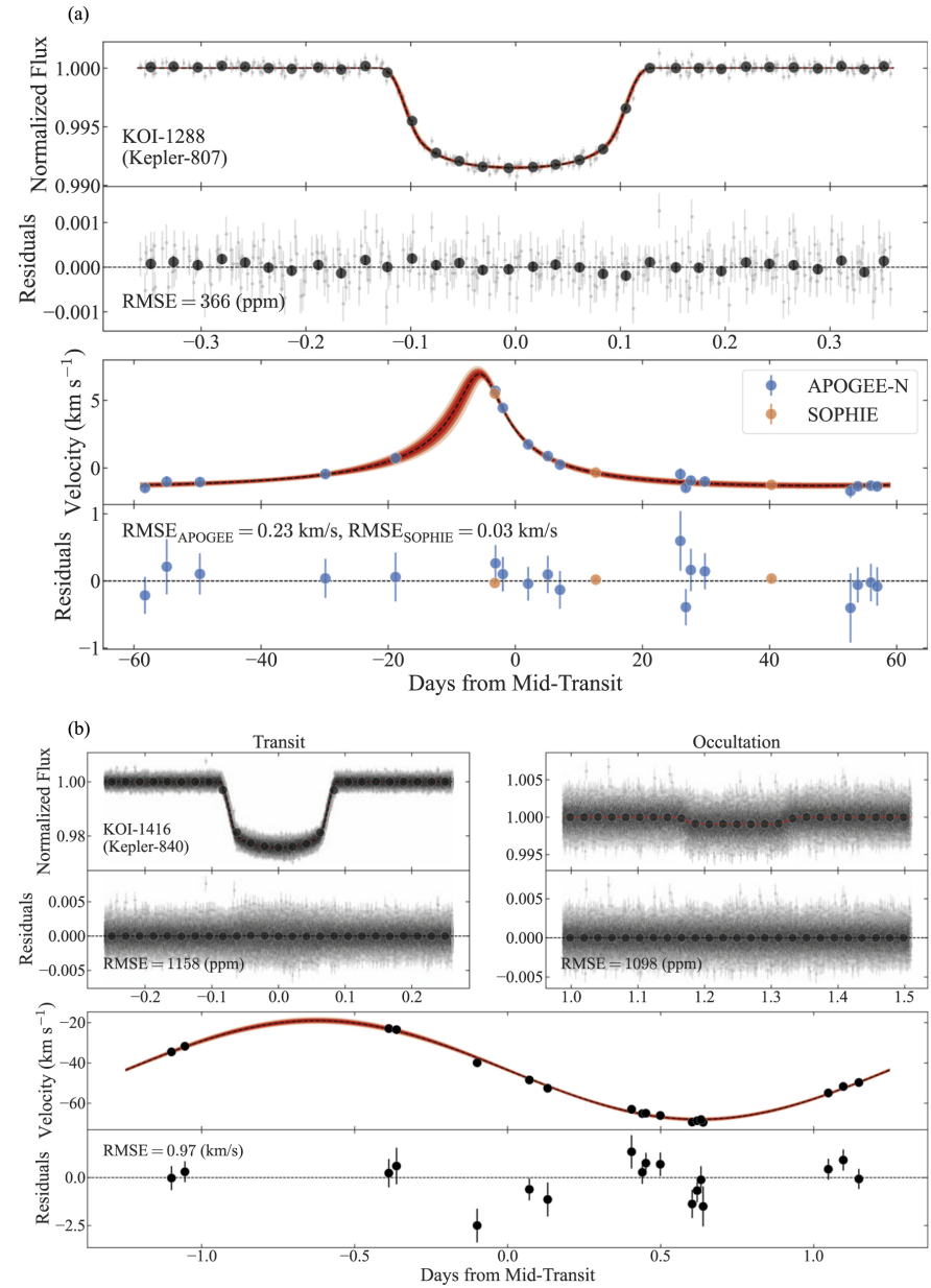
Figure 2. Photometry and RVs for the sample of 28 KOIs from Caleb I. Cañas et al 2023 Astrophys. J. Suppl. 265 doi:10.3847/1538-4365/acbcbe https://dx.doi.org/10.3847/1538-4365/acbcbe © 2023. The Author(s). Published by the American Astronomical Society.
