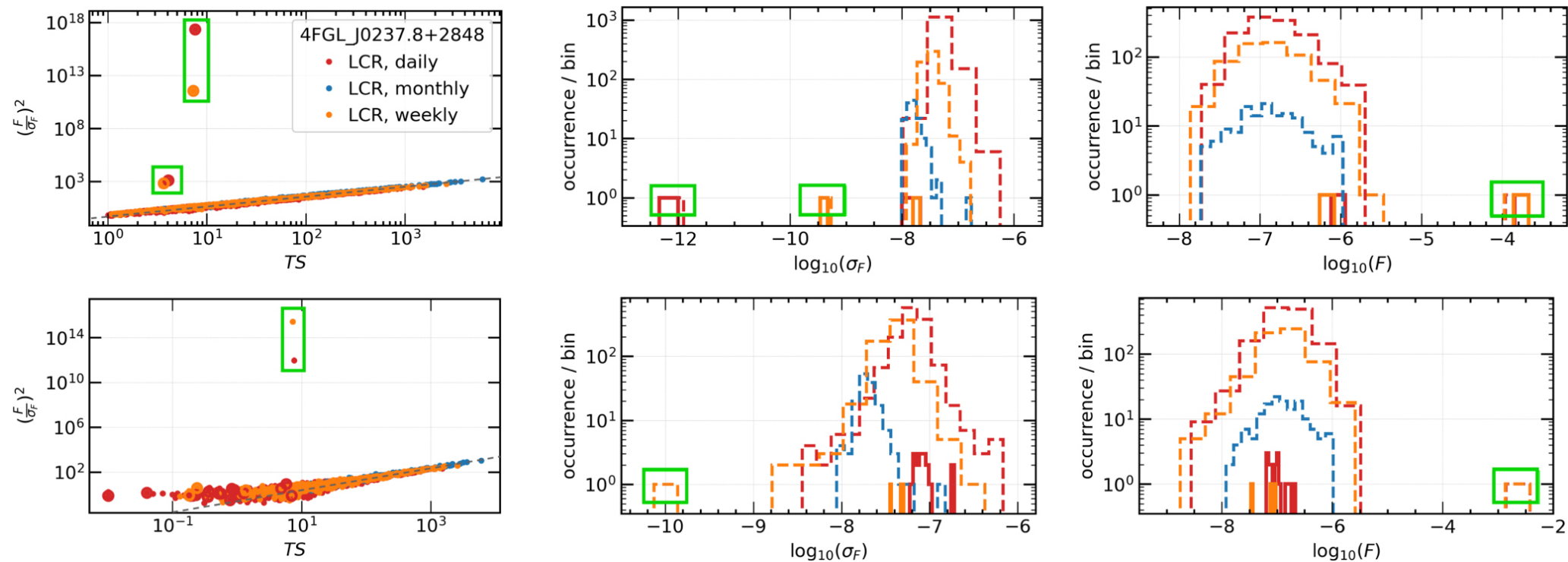
Figure 8. from S. Abdollahi et al 2023 Astrophys. J. Suppl. 265 doi:10.3847/1538-4365/acbb6a https://dx.doi.org/10.3847/1538-4365/acbb6a © 2023. The Author(s). Published by the American Astronomical Society.
